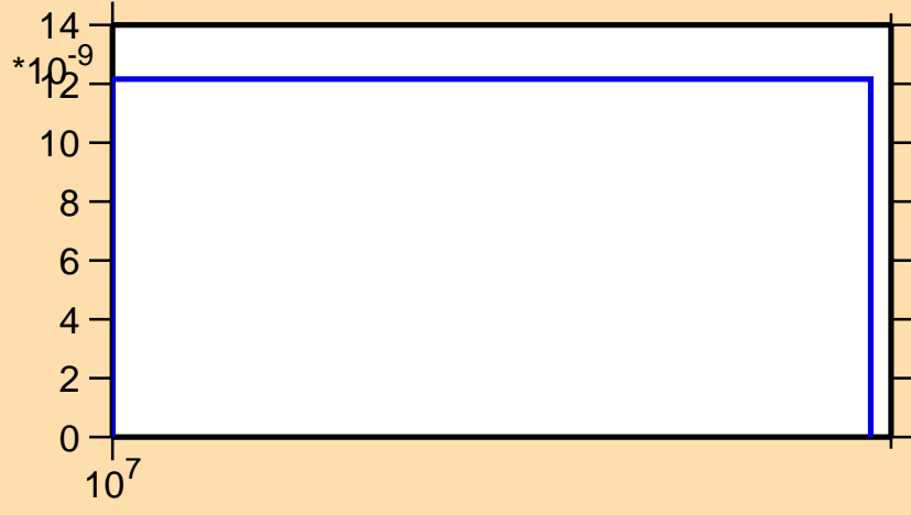
\sigma vs. E for ^{152}\text{Dy}(n,3n\alpha)
