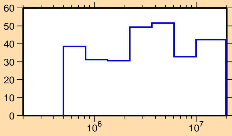
\Delta\sigma/\sigma vs. E for ^{152}\text{Dy}(n,n_1)
