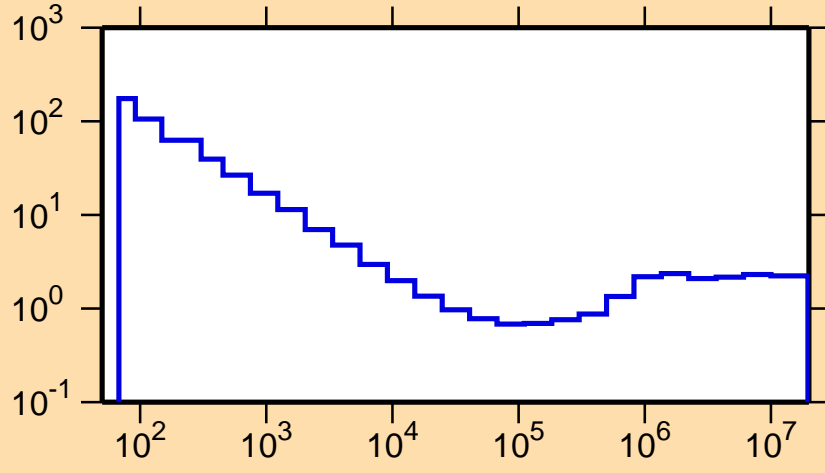
\sigma vs. E for ^{152}\text{Dy}(n,\text{nonel.})
