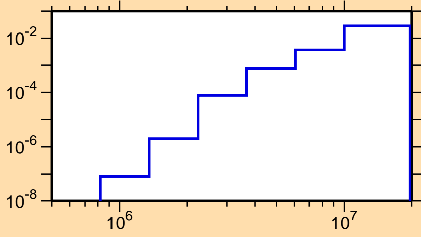
\sigma vs. E for ^{152}\text{Dy}(n,p)
