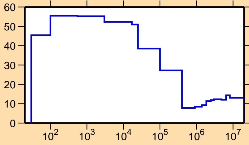
\Delta\sigma/\sigma vs. E for ^{152}\text{Dy}(n,el.)
