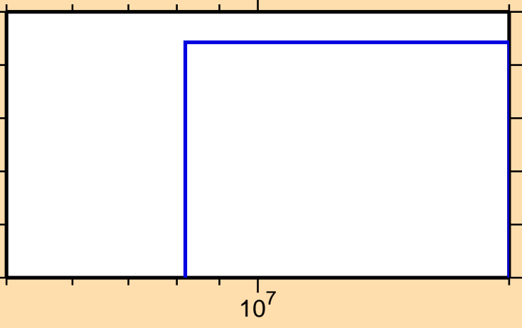
\sigma vs. E for ^{152}\text{Dy} (mt 45)
