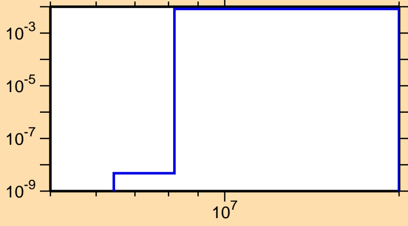
\sigma vs. E for ^{152}\text{Dy}(n,np)
