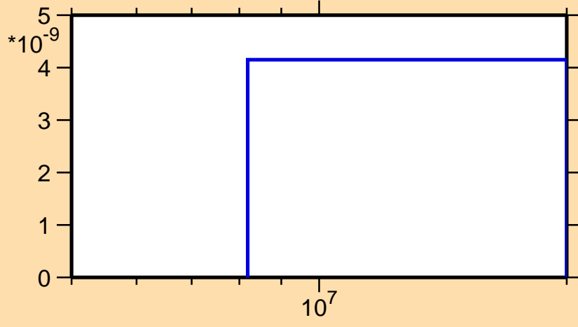
\sigma vs. E for ^{152}\text{Dy}(\text{mt117})
