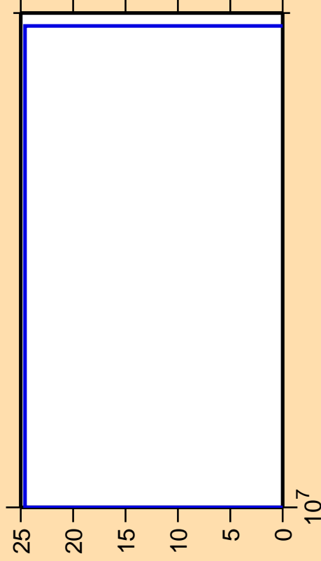
\Delta\sigma/\sigma vs. E for ^{153}\text{Dy}(n,3n\alpha)
