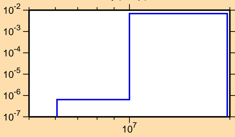
\sigma vs. E for ^{153}\text{Dy}(n,np)
