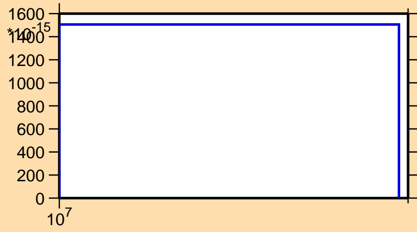
\sigma vs. E for ^{153}\text{Dy} (mt 34)
