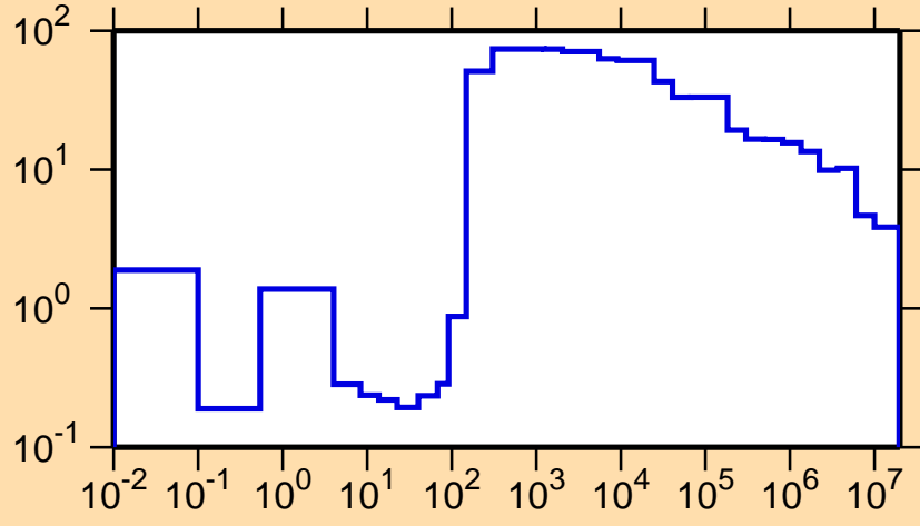
\Delta\sigma/\sigma vs. E for ^{153}\text{Dy}(n,\text{tot.})
