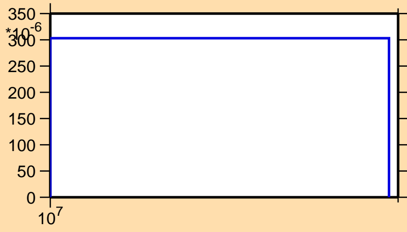
\sigma vs. E for ^{153}\text{Dy}(n,3n)
