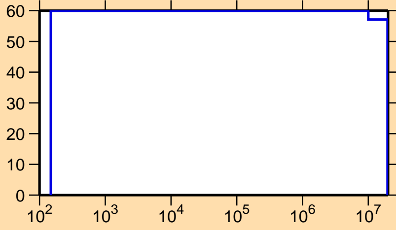
\Delta\sigma/\sigma vs. E for ^{153}\text{Dy}(n,p)
