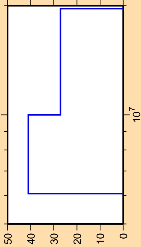
\Delta\sigma/\sigma vs. E for ^{153}\text{Dy}(n,2n)
