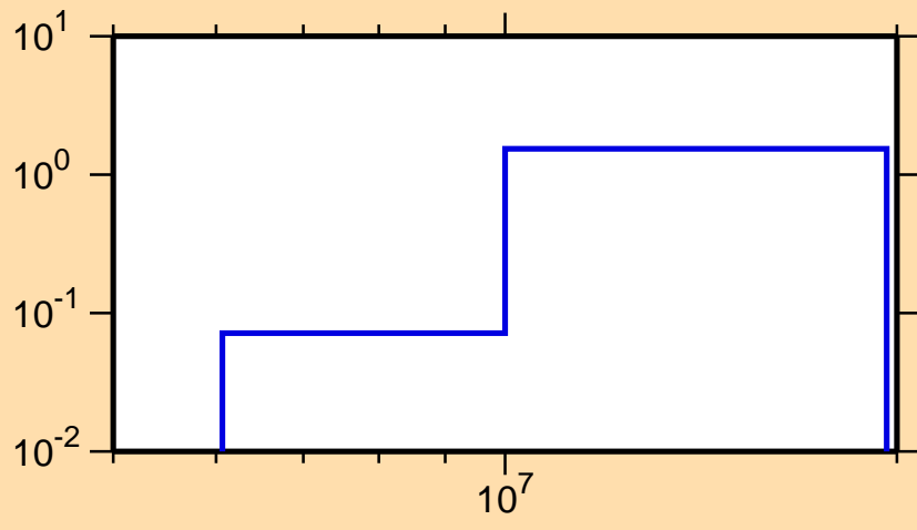
\sigma vs. E for ^{153}\text{Dy}(n,2n)
