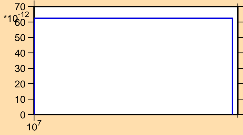
\sigma vs. E for ^{153}\text{Dy}(n,nt)
