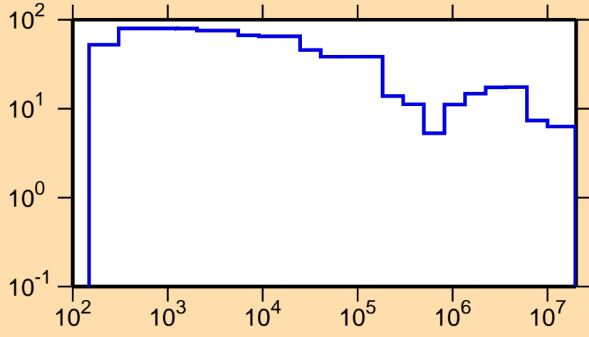
\Delta\sigma/\sigma vs. E for ^{153}\text{Dy}(n,\text{el.})
