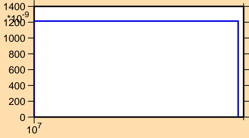
\sigma vs. E for ^{153}\text{Dy}(n,2np)
