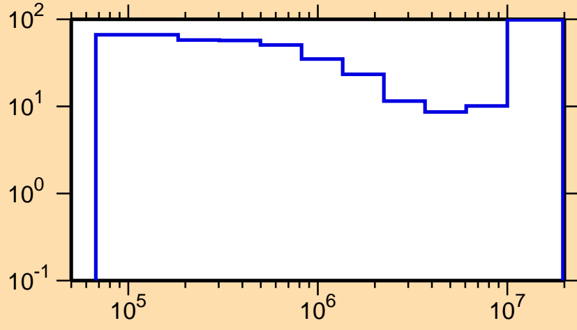
\Delta\sigma/\sigma vs. E for ^{153}\text{Dy}(n,\text{inel.})
