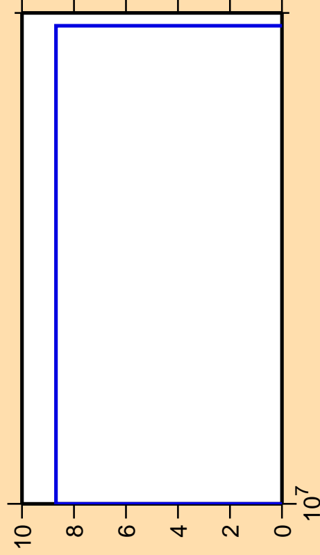
\Delta\sigma/\sigma vs. E for ^{153}\text{Dy} (mt 34)
