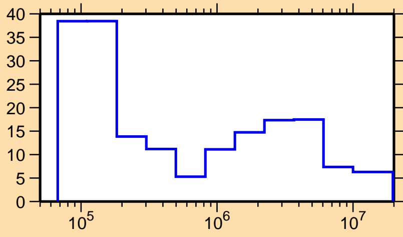
\Delta\sigma/\sigma vs. E for ^{153}\text{Dy}(n,\text{el.})
