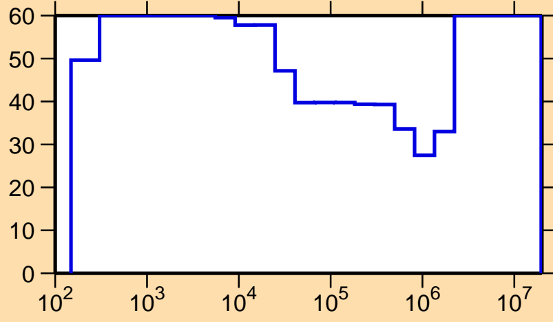
\Delta\sigma/\sigma vs. E for ^{153}\text{Dy}(n,\gamma)
