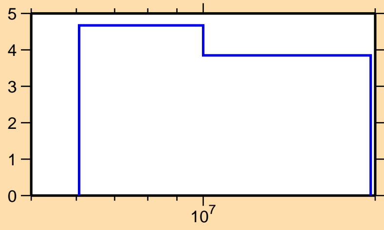
\Delta\sigma/\sigma vs. E for ^{153}\text{Dy}(n,\text{tot.})
