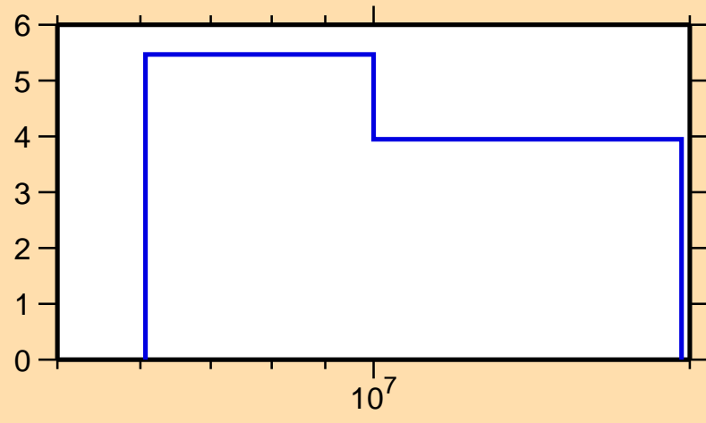
\Delta\sigma/\sigma vs. E for ^{153}\text{Dy}(n,\text{nonel.})
