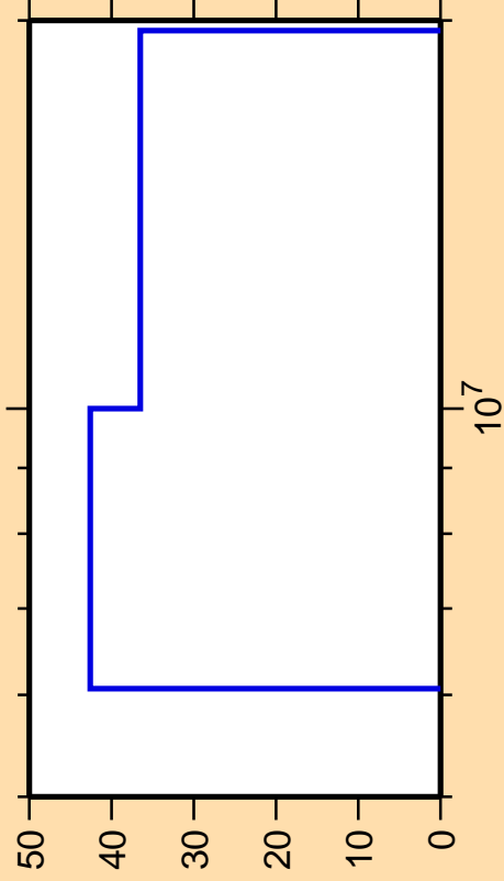
\Delta\sigma/\sigma vs. E for ^{153}\text{Dy}(n,n_1)
