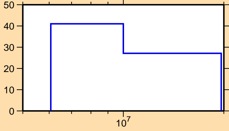
\Delta\sigma/\sigma vs. E for ^{153}\text{Dy}(n,2n)
