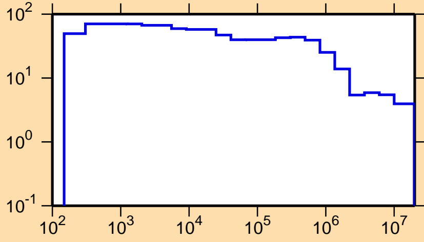
\Delta\sigma/\sigma vs. E for ^{153}\text{Dy}(n,\text{nonel.})
