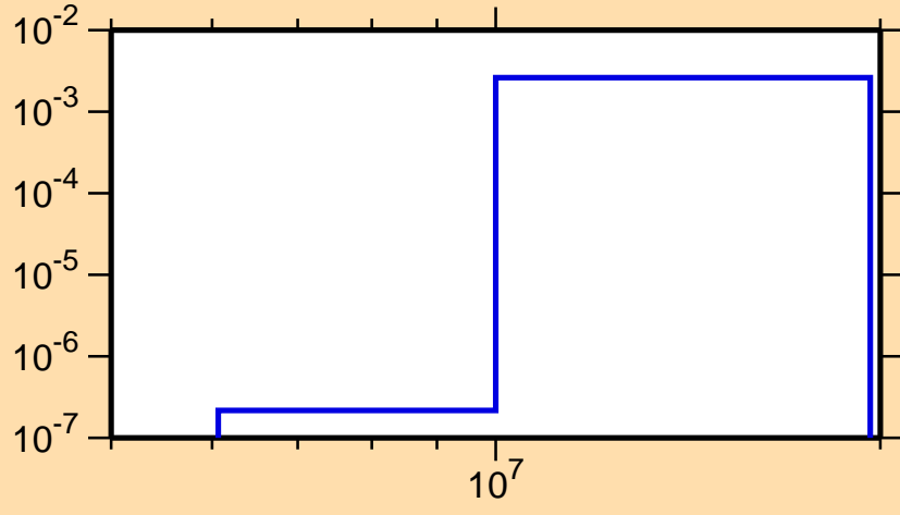
\sigma vs. E for ^{153}\text{Dy}(n,d)
