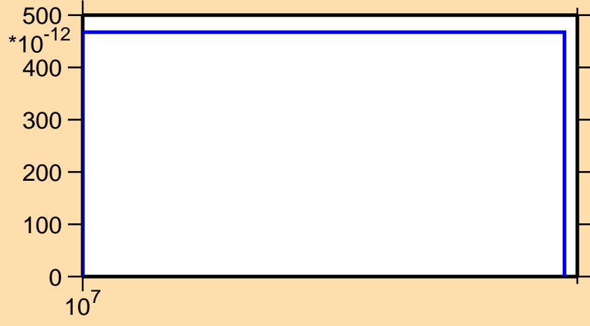
\sigma vs. E for ^{153}\text{Dy}(\text{mt117})
