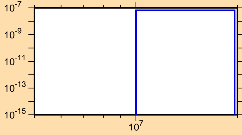
\sigma vs. E for ^{153}\text{Dy}(n,\text{He3})
