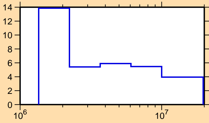
\Delta\sigma/\sigma vs. E for ^{153}\text{Dy}(n,\text{nonel.})
