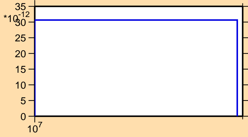
\sigma vs. E for ^{153}\text{Dy}(n,pt)
