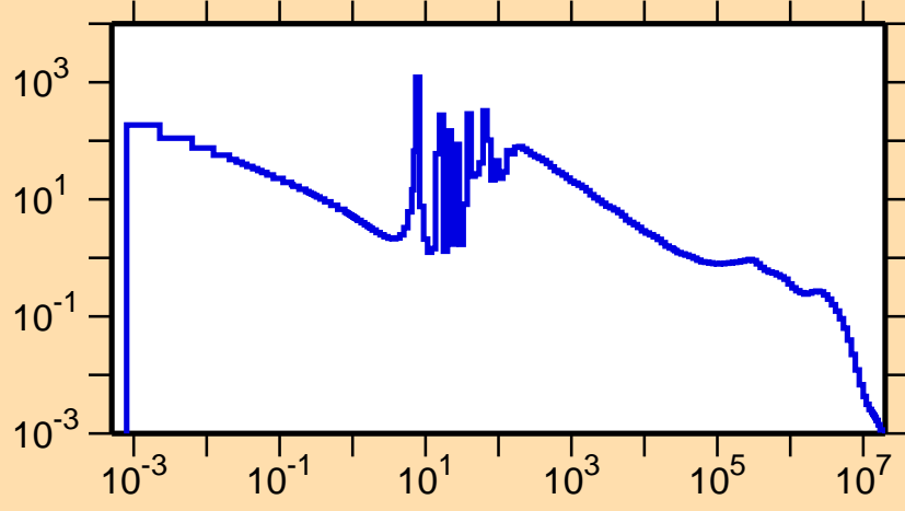
\sigma vs. E for ^{154}\text{Dy}(n,\gamma)
