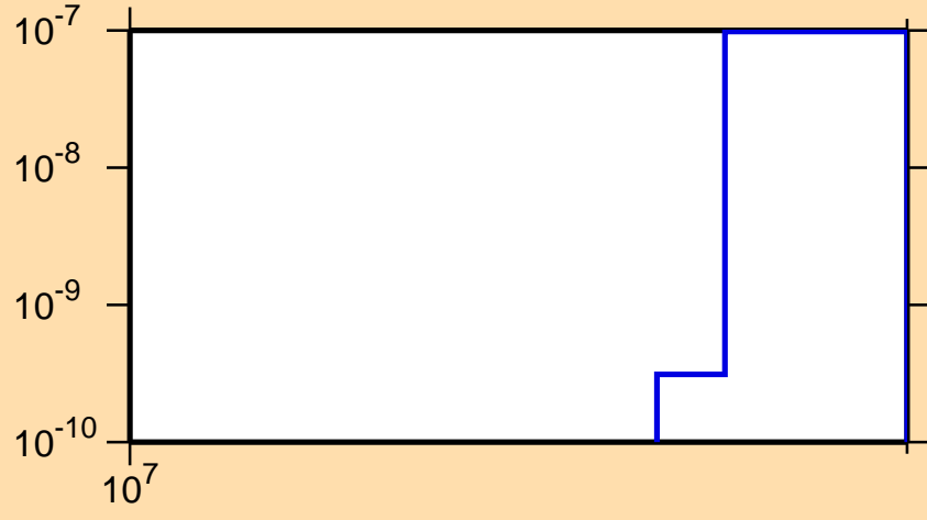
\sigma vs. E for ^{154}\text{Dy}(n,\text{nd})
