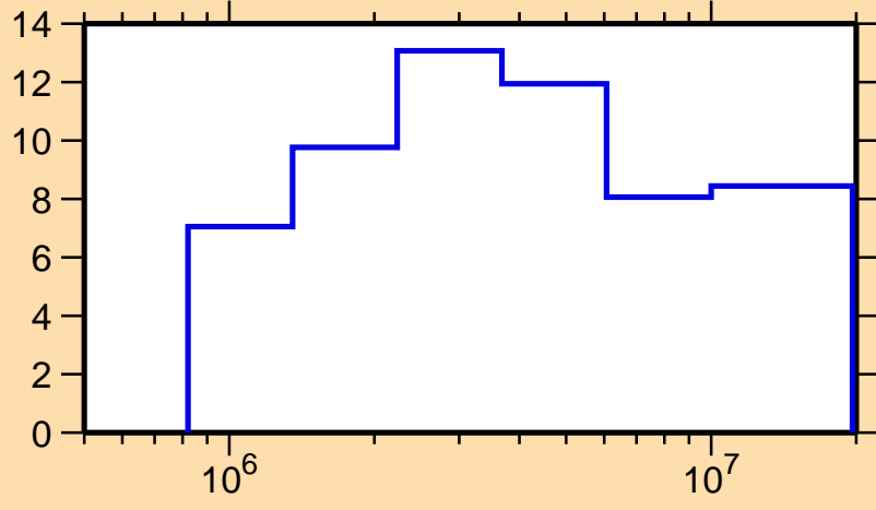
\Delta\sigma/\sigma vs. E for ^{154}\text{Dy}(n,el.)
