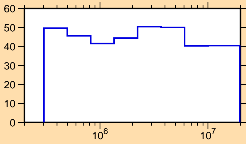
\Delta\sigma/\sigma vs. E for ^{154}\text{Dy}(n,n_1)
