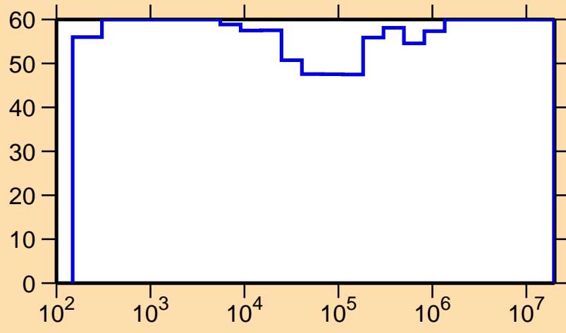
\Delta\sigma/\sigma vs. E for ^{154}\text{Dy}(n,\gamma)
