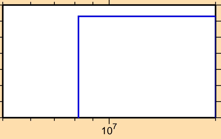
\sigma vs. E for ^{154}\text{Dy}(n,2n\alpha)
