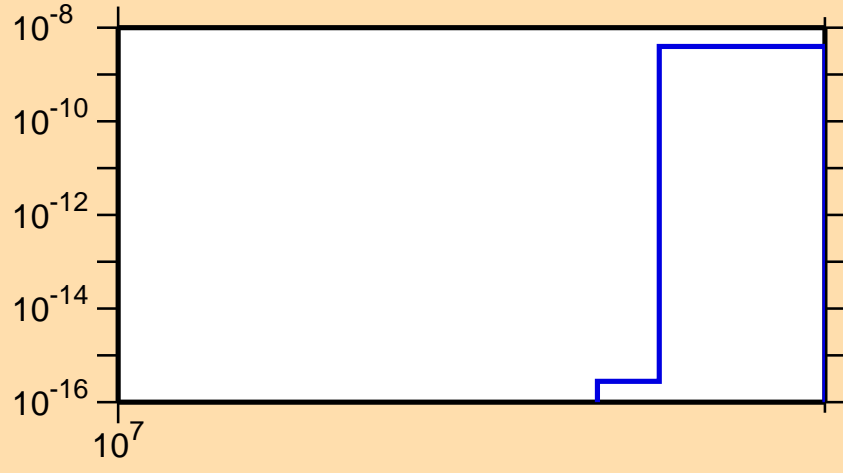
\sigma vs. E for ^{155}\text{Dy}(n,3n\alpha)
