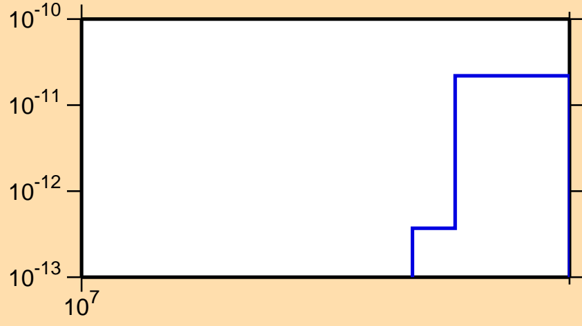
\sigma vs. E for ^{155}\text{Dy}(n,pd)
