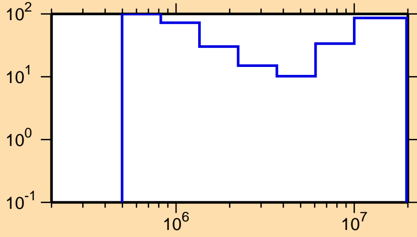
\Delta\sigma/\sigma vs. E for ^{155}\text{Dy}(n,n\text{cont.})
