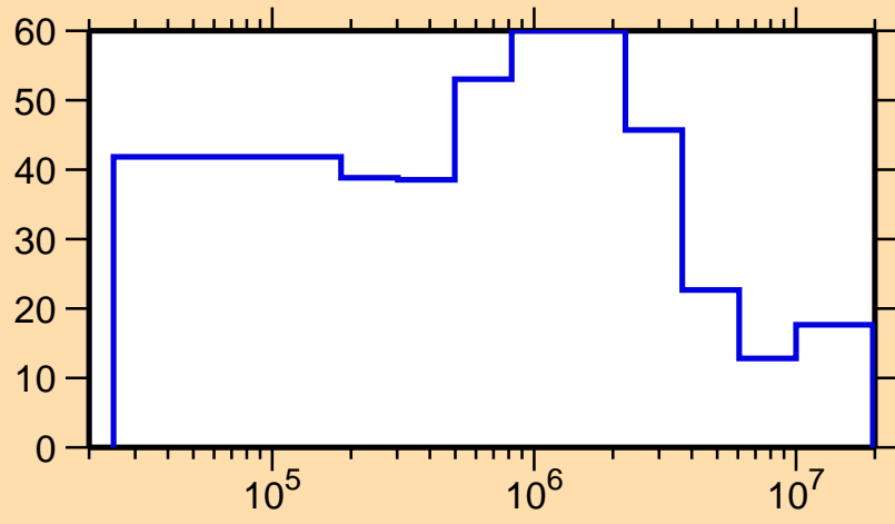
\Delta\sigma/\sigma vs. E for ^{155}\text{Dy}(n,n_1)
