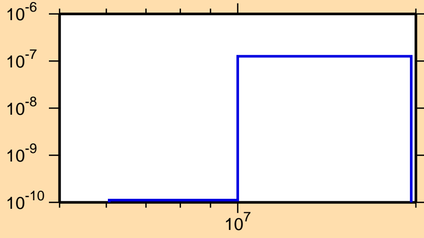
\sigma vs. E for ^{155}\text{Dy}(n,p\alpha)
