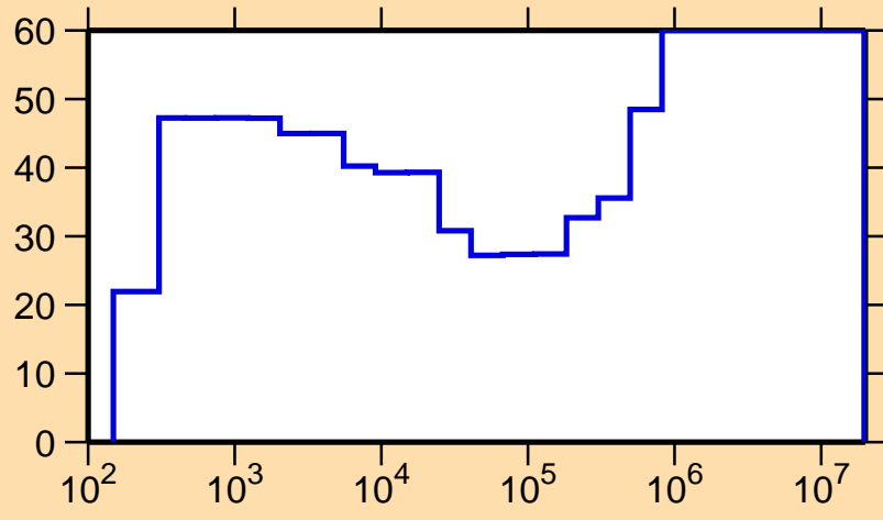
\Delta\sigma/\sigma vs. E for ^{155}\text{Dy}(n,\gamma)
