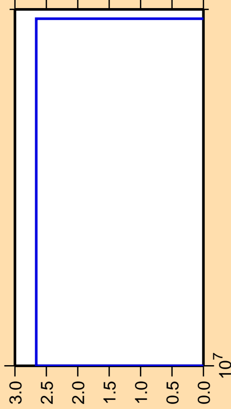
\Delta\sigma/\sigma vs. E for ^{155}\text{Dy}(n,pt)
