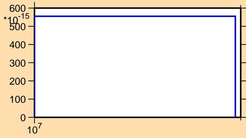
\sigma vs. E for ^{155}\text{Dy}(n,pt)
