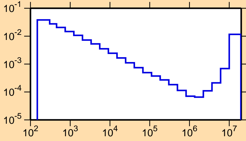
\sigma vs. E for ^{155}\text{Dy}(n,\alpha)
