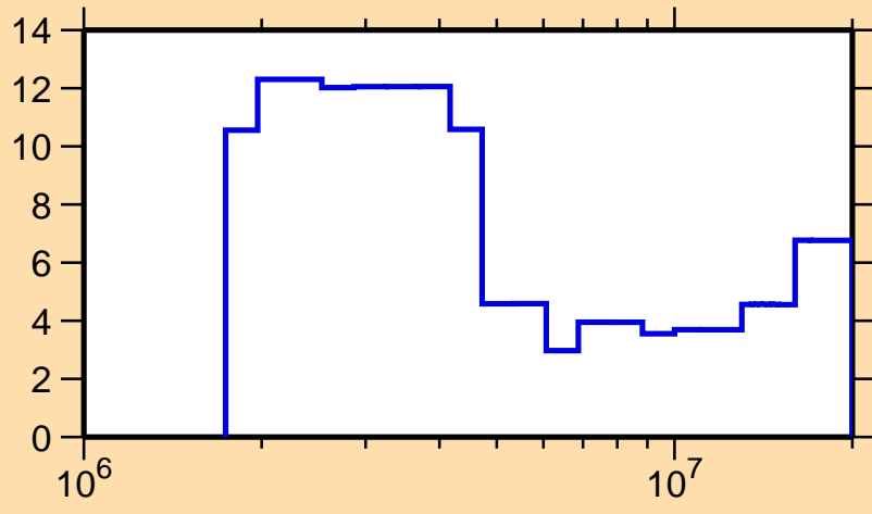
\Delta\sigma/\sigma vs. E for ^{156}\text{Dy}(n,el.)
