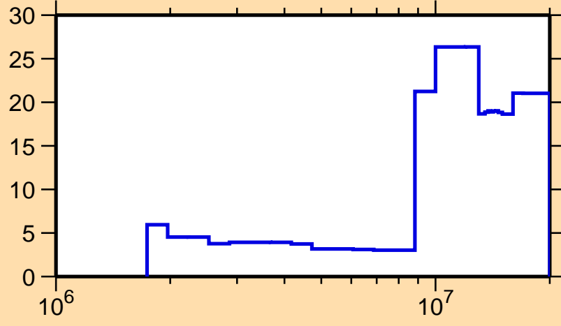
\Delta\sigma/\sigma vs. E for ^{156}\text{Dy}(n,inel.)
