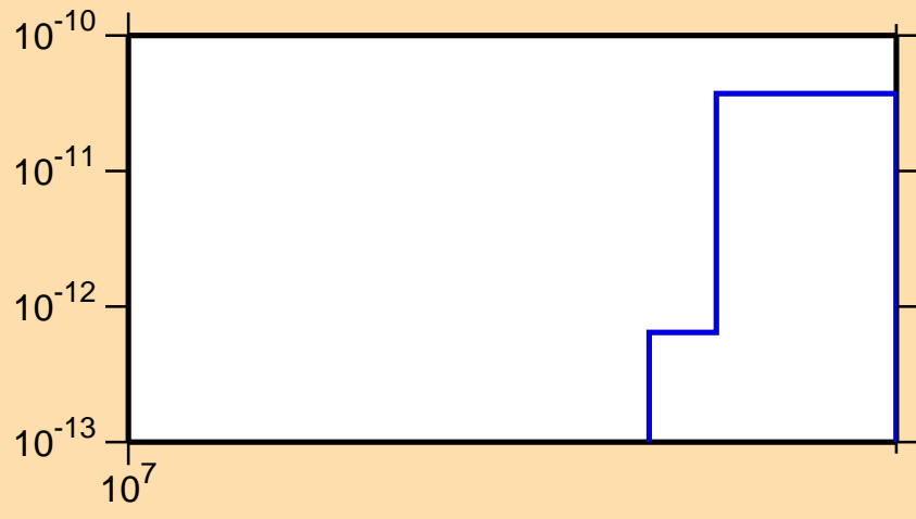
\sigma vs. E for ^{156}\text{Dy} (mt 45)
