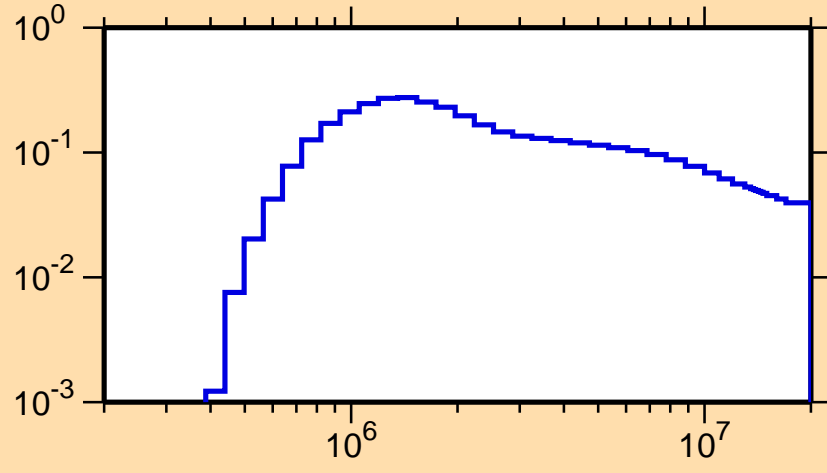
\sigma vs. E for ^{156}\text{Dy}(n,n_2)
