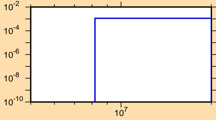
\sigma vs. E for ^{156}\text{Dy}(n,np)
