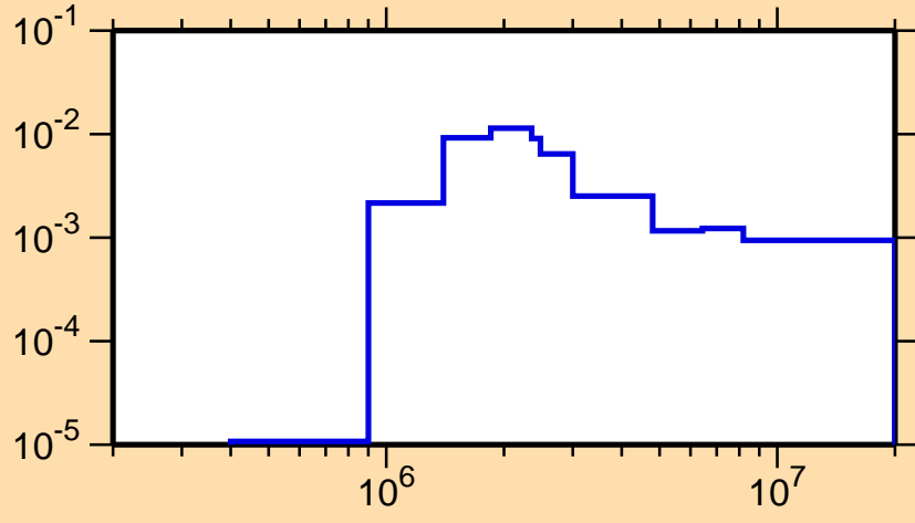
\sigma vs. E for ^{156}\text{Dy}(n,n_4)
