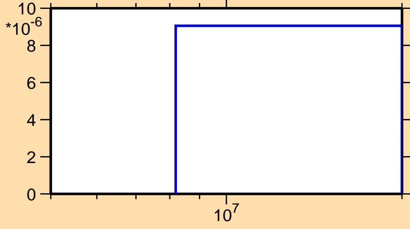
\sigma vs. E for ^{156}\text{Dy}(n,t)
