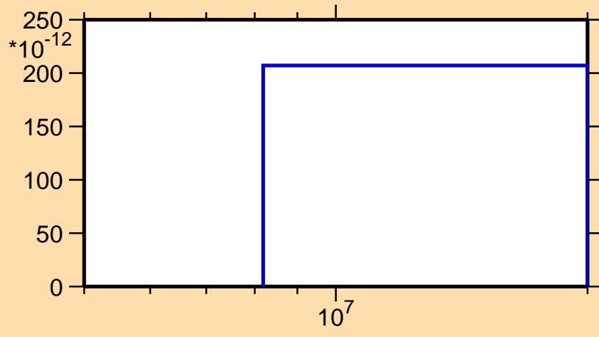
\sigma vs. E for ^{156}\text{Dy}(n,p\alpha)
