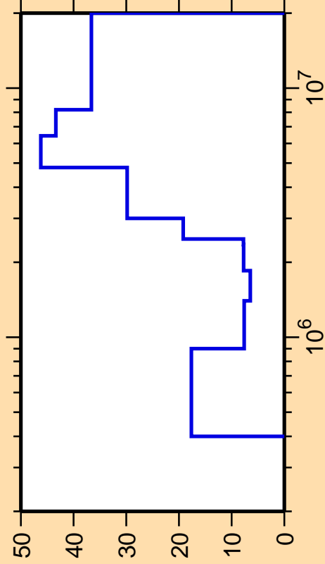
\Delta\sigma/\sigma vs. E for ^{156}\text{Dy}(n,n_4)
