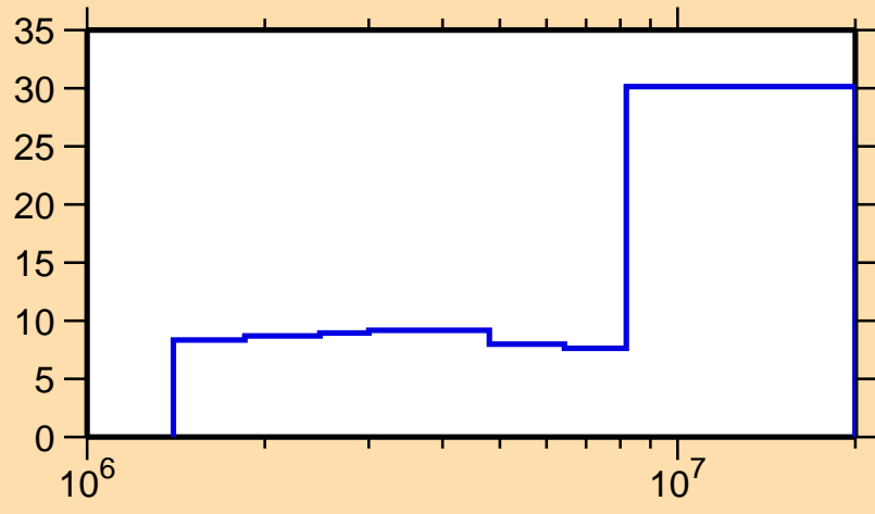
\Delta\sigma/\sigma vs. E for ^{156}\text{Dy}(n,n\text{cont.})
