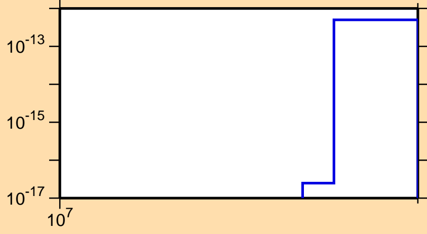
\sigma vs. E for ^{157}\text{Dy}(n,3n\alpha)
