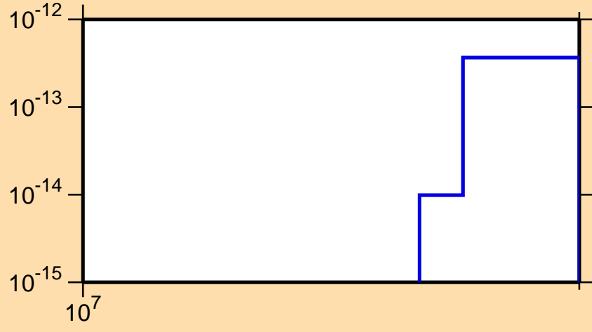
\sigma vs. E for ^{157}\text{Dy} (mt 45)
