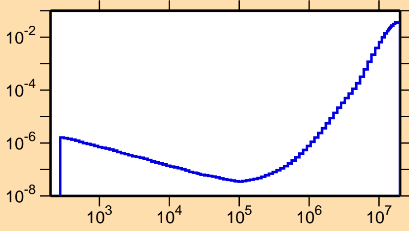
\sigma vs. E for ^{157}\text{Dy}(n,p)
