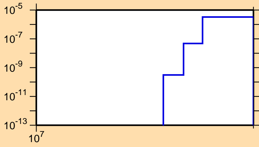
\sigma vs. E for ^{157}\text{Dy}(n,2np)
