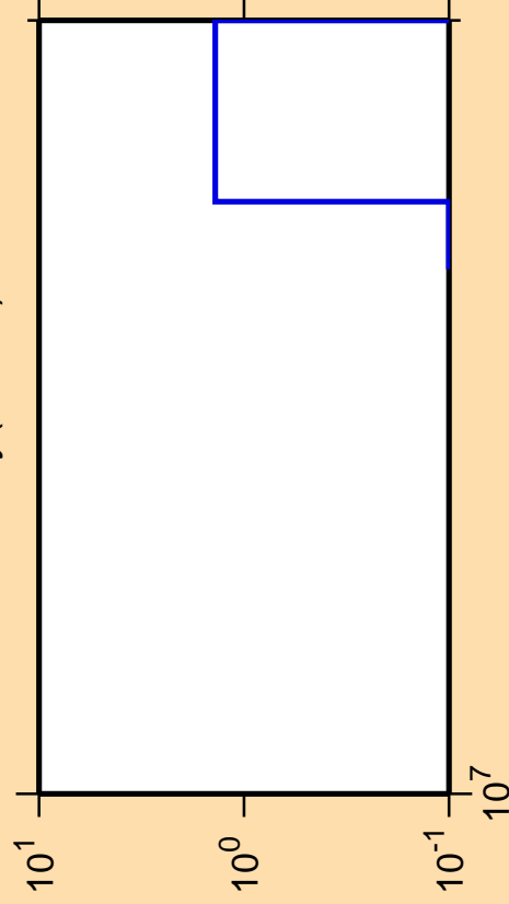
\Delta\sigma/\sigma vs. E for ^{157}\text{Dy} (mt 45)
