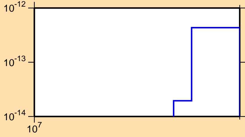
\sigma vs. E for ^{157}\text{Dy}(\text{mt117})
