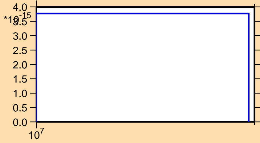
\sigma vs. E for ^{157}\text{Dy} (mt 45)
