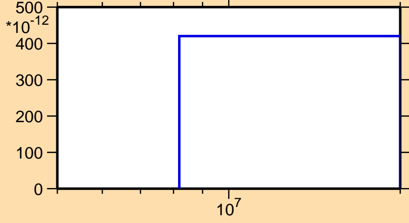
\sigma vs. E for ^{157}\text{Dy}(n,\text{He}3)
