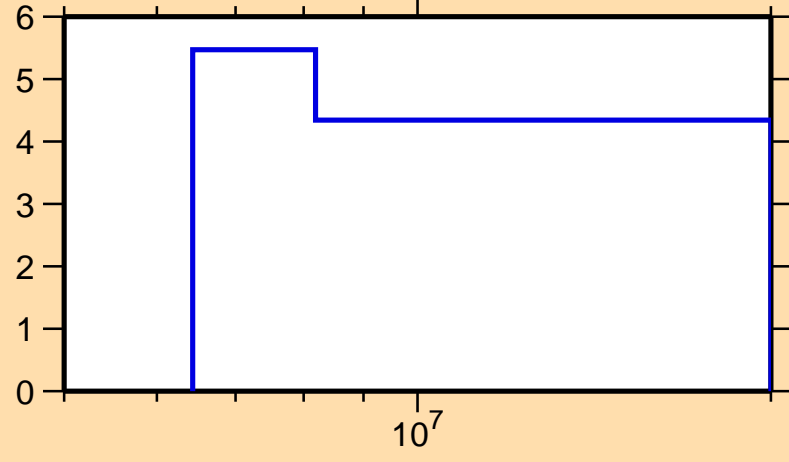
\Delta\sigma/\sigma vs. E for ^{157}\text{Dy}(n,\text{nonel.})
