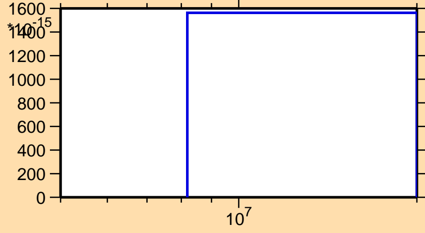
\sigma vs. E for ^{157}\text{Dy}(n,nt)
