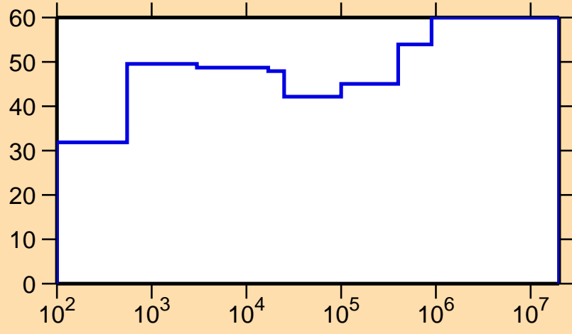
\Delta\sigma/\sigma vs. E for ^{157}\text{Dy}(n,\gamma)
