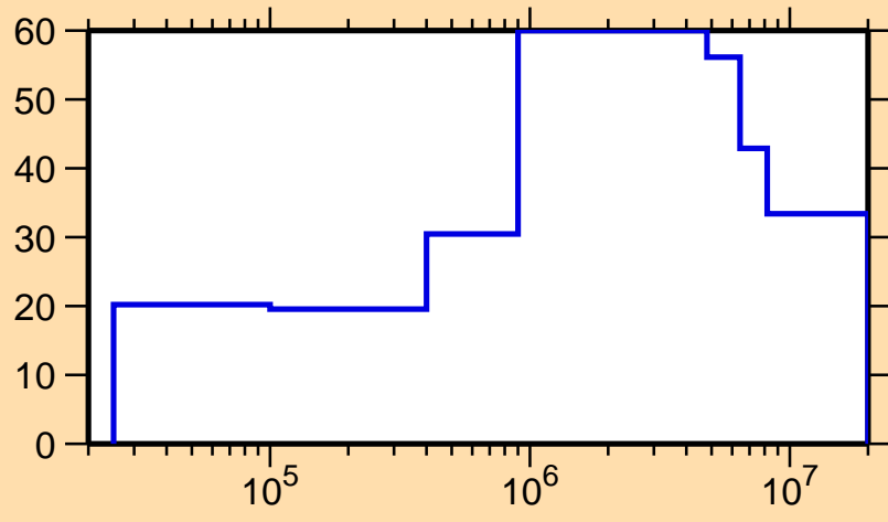
\Delta\sigma/\sigma vs. E for ^{157}\text{Dy}(n,n_1)
