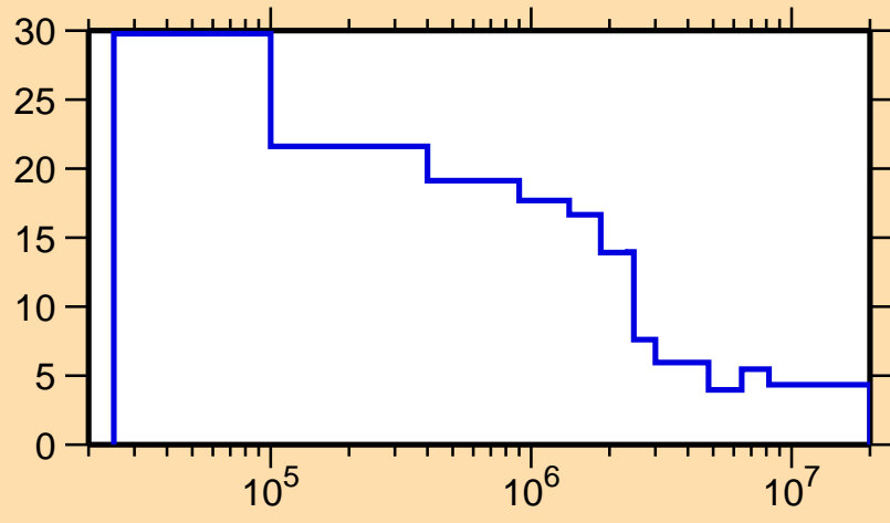
\Delta\sigma/\sigma vs. E for ^{157}\text{Dy}(n,\text{nonel.})
