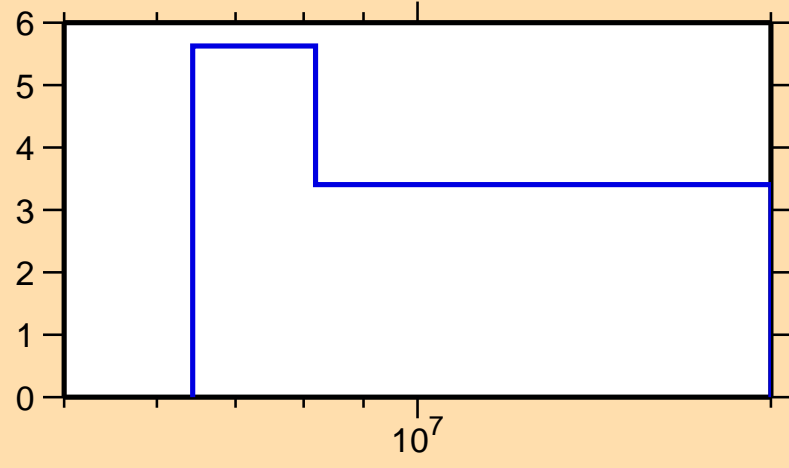
\Delta\sigma/\sigma vs. E for ^{157}\text{Dy}(n,\text{el.})
