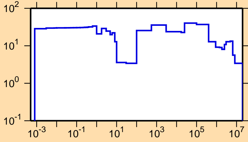
\Delta\sigma/\sigma vs. E for ^{157}\text{Dy}(n,\text{el.})
