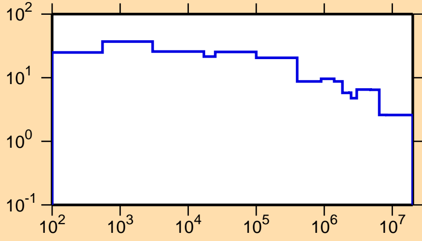
\Delta\sigma/\sigma vs. E for ^{157}\text{Dy}(n,\text{tot.})
