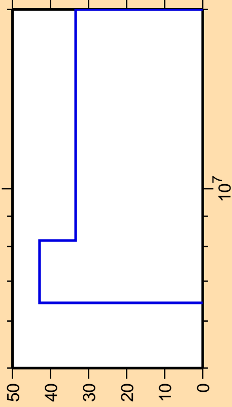
\Delta\sigma/\sigma vs. E for ^{157}\text{Dy}(n,n_1)
