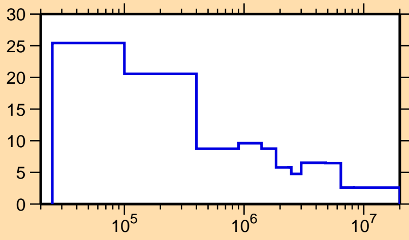
\Delta\sigma/\sigma vs. E for ^{157}\text{Dy}(n,\text{tot.})
