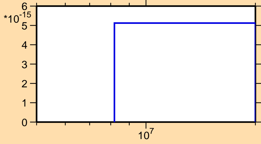
\sigma vs. E for ^{157}\text{Dy}(n,\text{pt})
