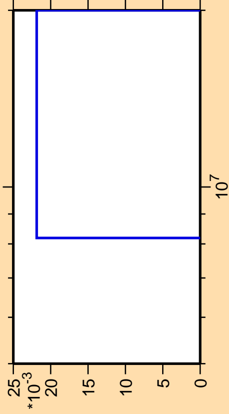
\Delta\sigma/\sigma vs. E for ^{157}\text{Dy}(n,pd)
