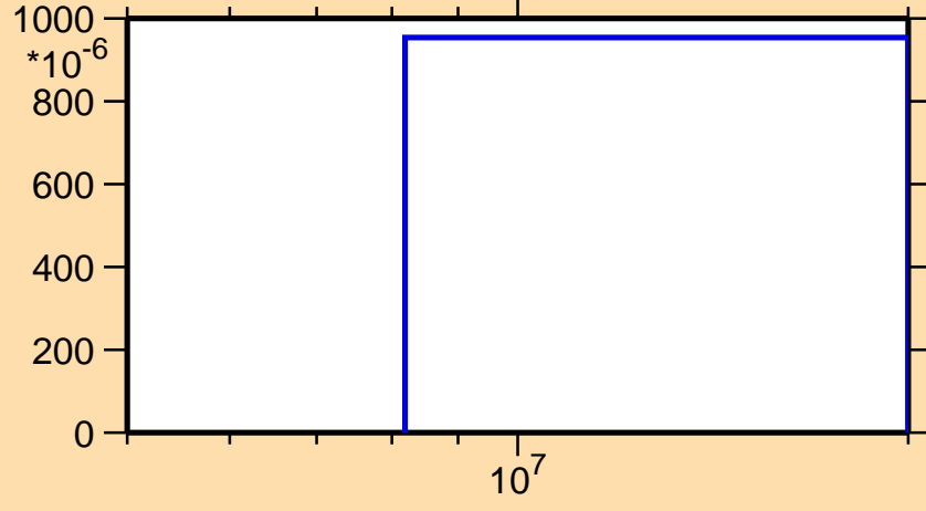
\sigma vs. E for ^{157}\text{Dy}(n,3n)
