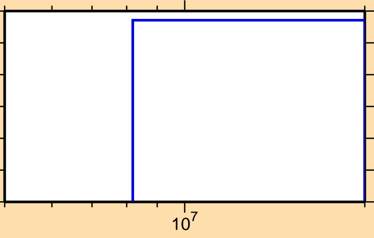
\sigma vs. E for ^{157}\text{Dy}(n,2np)
