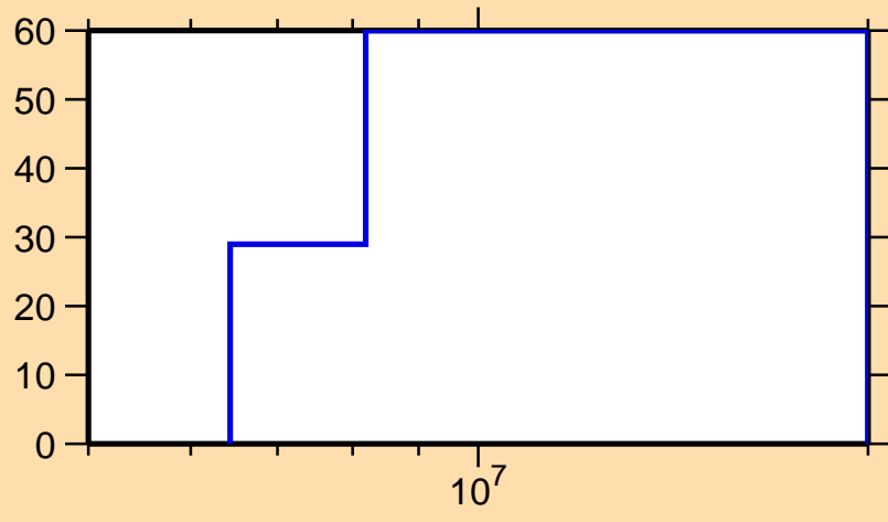
\Delta\sigma/\sigma vs. E for ^{157}\text{Dy}(n,\text{inel.})
