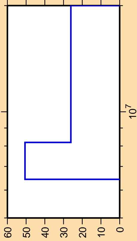
\Delta\sigma/\sigma vs. E for ^{157}\text{Dy}(n,2n)
