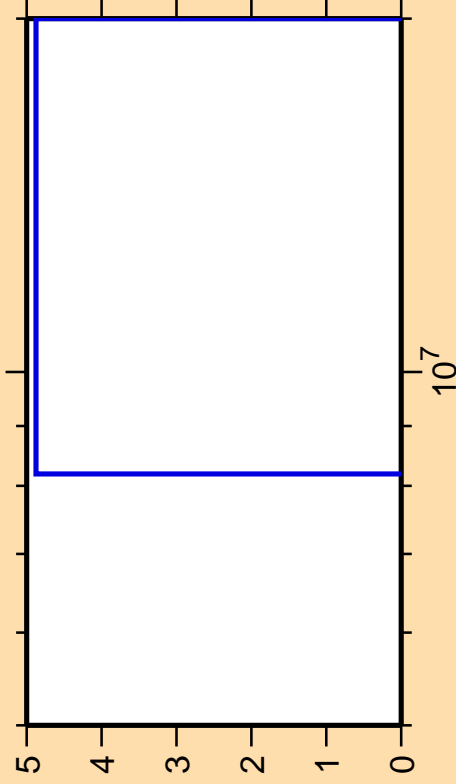
\Delta\sigma/\sigma vs. E for ^{157}\text{Dy}(n,nt)
