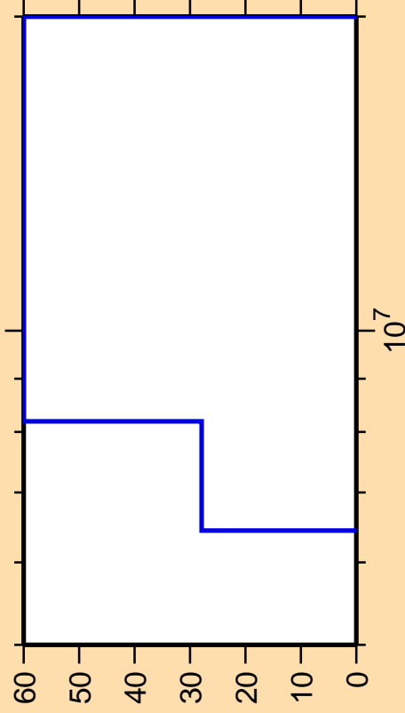
\Delta\sigma/\sigma vs. E for ^{157}\text{Dy}(n,n\text{cont.})
