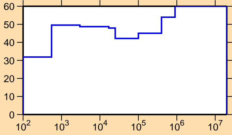
\Delta\sigma/\sigma vs. E for ^{157}\text{Dy}(n,\gamma)
