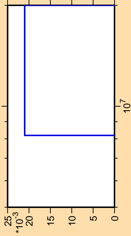
\Delta\sigma/\sigma vs. E for ^{157}\text{Dy}(\text{mt117})
