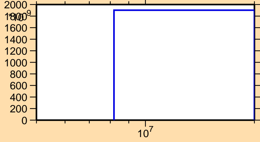
\sigma vs. E for ^{157}\text{Dy}(n,2n\alpha)
