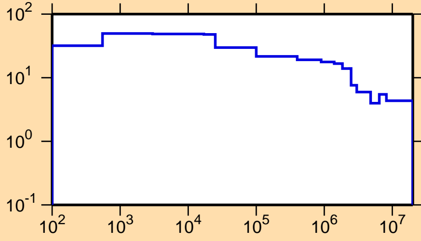
\Delta\sigma/\sigma vs. E for ^{157}\text{Dy}(n,\text{nonel.})
