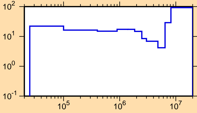
\Delta\sigma/\sigma vs. E for ^{157}\text{Dy}(n,\text{inel.})
