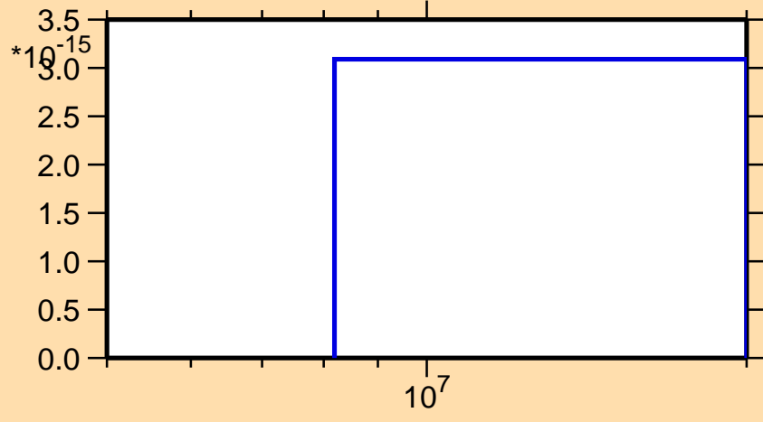
\sigma vs. E for ^{157}\text{Dy}(n,pd)
