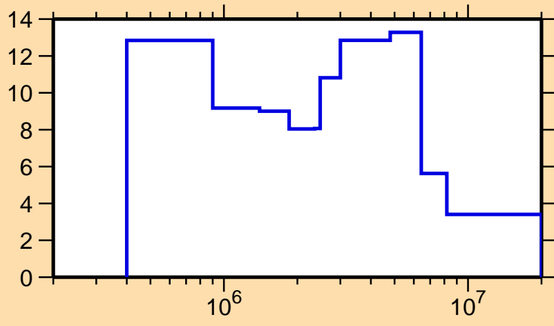
\Delta\sigma/\sigma vs. E for ^{157}\text{Dy}(n,\text{el.})
