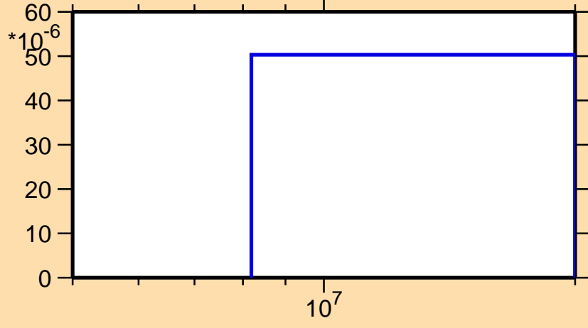
\sigma vs. E for ^{157}\text{Dy}(n,t)
