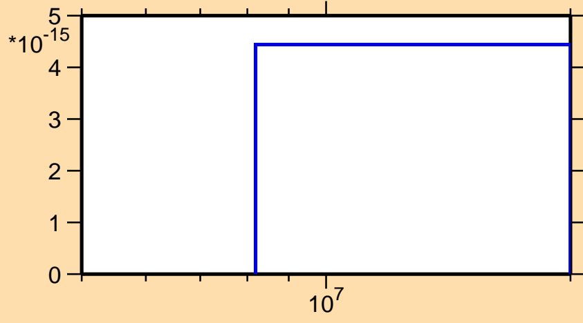
\sigma vs. E for ^{157}\text{Dy}(\text{mt117})
