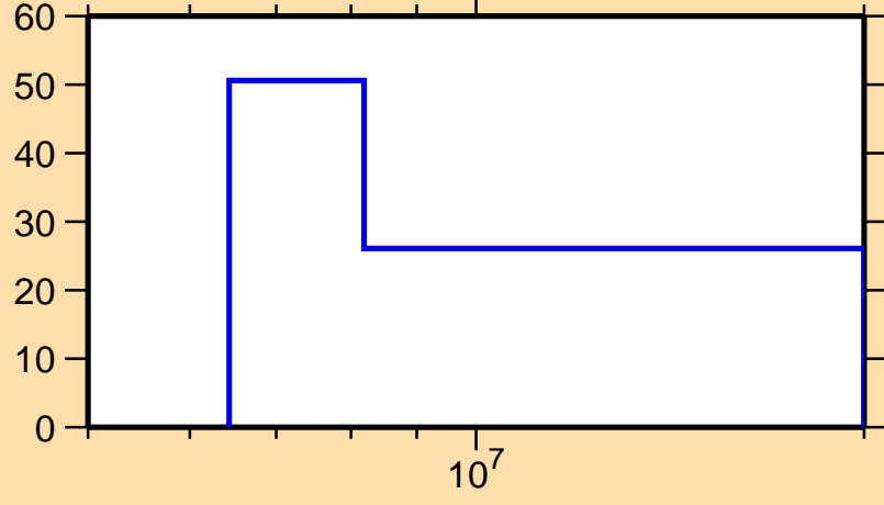
\Delta\sigma/\sigma vs. E for ^{157}\text{Dy}(n,2n)
