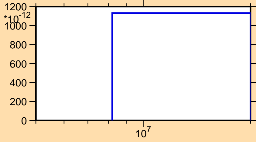
\sigma vs. E for ^{157}\text{Dy}(n,p\alpha)
