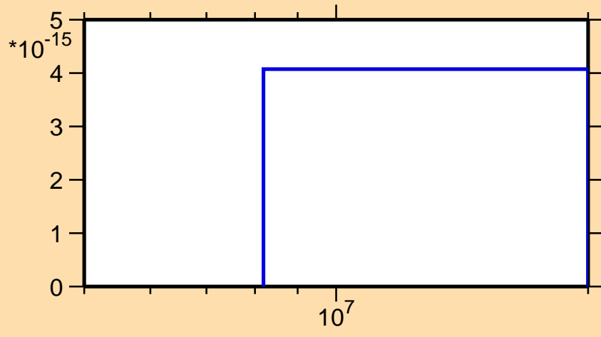
\sigma vs. E for ^{157}\text{Dy}(n,3n\alpha)
