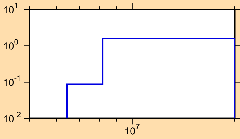
\sigma vs. E for ^{157}\text{Dy}(n,2n)
