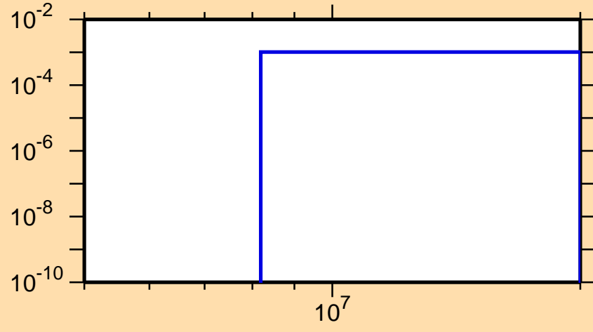
\sigma vs. E for ^{157}\text{Dy}(n,d)
