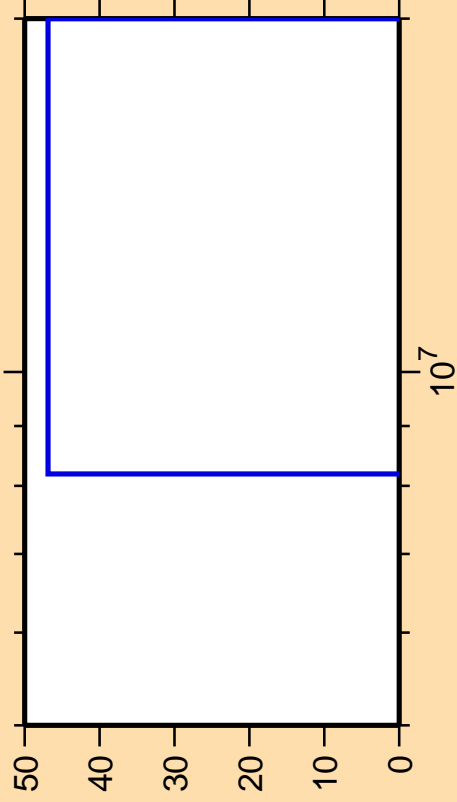
\Delta\sigma/\sigma vs. E for ^{157}\text{Dy}(n,3n)
