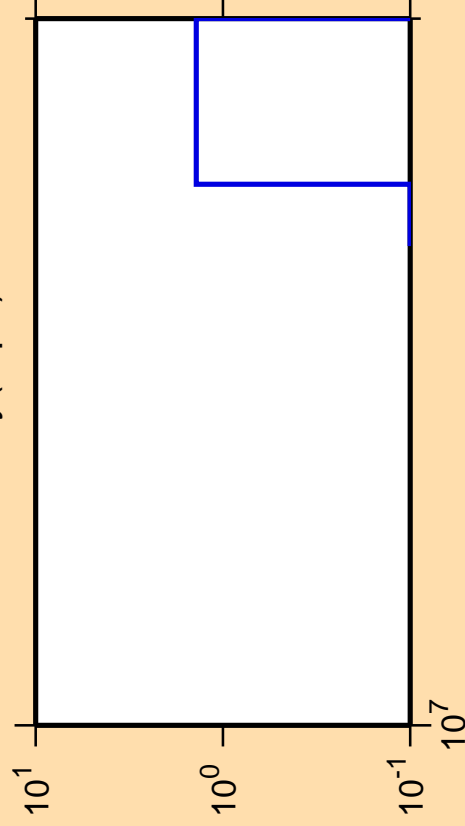
\Delta\sigma/\sigma vs. E for ^{158}\text{Dy}(n,\text{pd})
