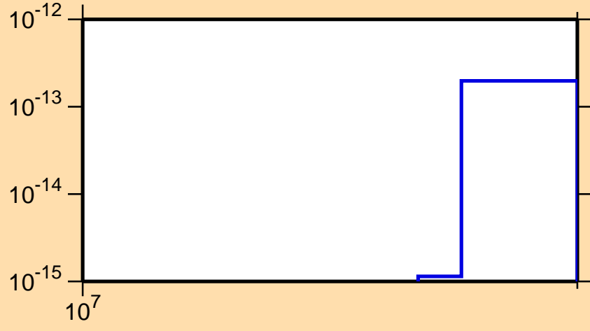
\sigma vs. E for ^{158}\text{Dy} (mt 45)
