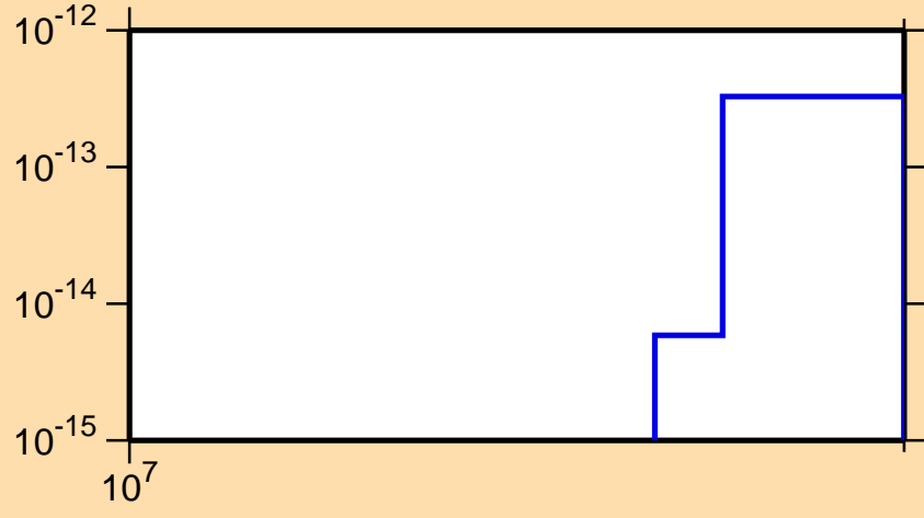
\sigma vs. E for ^{158}\text{Dy}(\text{mt117})
