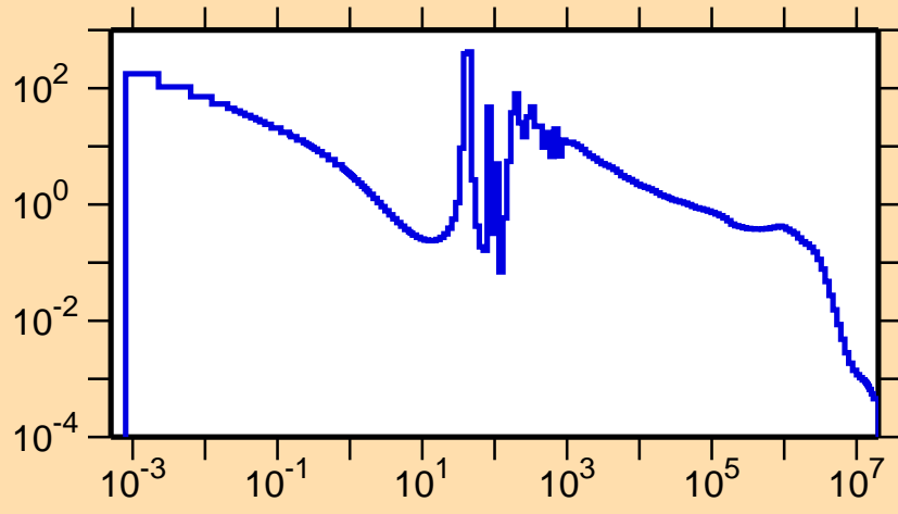
\sigma vs. E for ^{158}\text{Dy}(n,\gamma)
