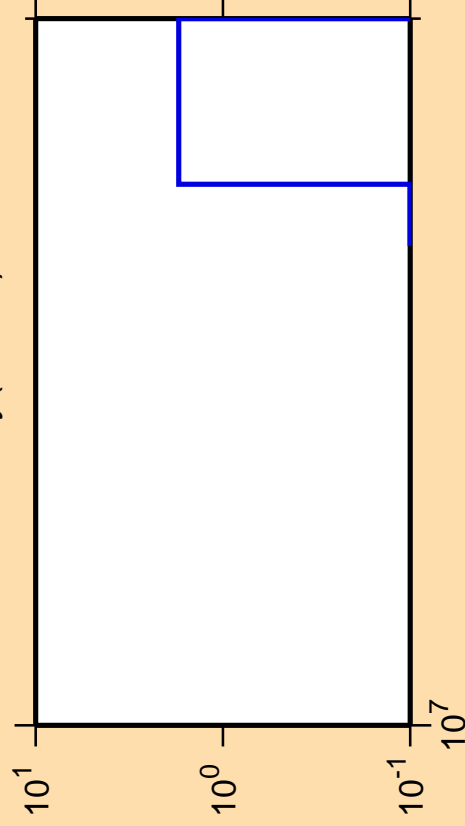
\Delta\sigma/\sigma vs. E for ^{158}\text{Dy} (mt 45)
