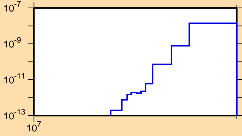
\sigma vs. E for ^{158}\text{Dy}(n,\text{He}3)
