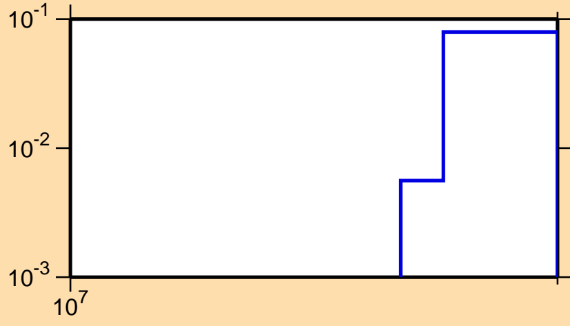
\sigma vs. E for ^{158}\text{Dy}(n,3n)
