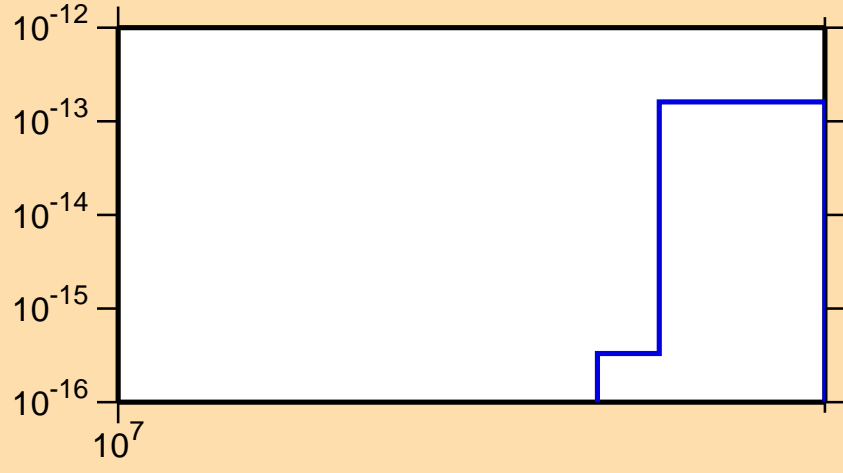
\sigma vs. E for ^{158}\text{Dy}(n,\text{pd})
