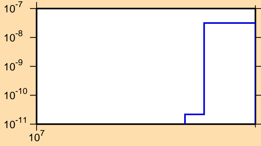
\sigma vs. E for ^{158}\text{Dy}(n,nd)
