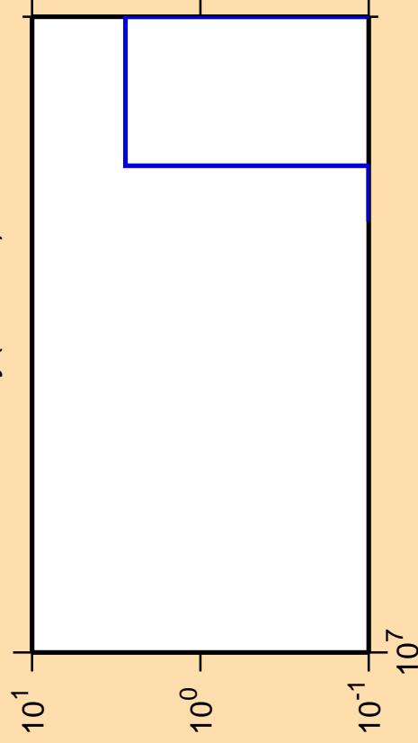
\Delta\sigma/\sigma vs. E for ^{158}\text{Dy}(\text{mt117})
