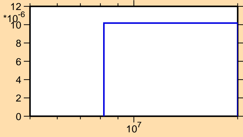
\sigma vs. E for ^{158}\text{Dy}(n,t)
