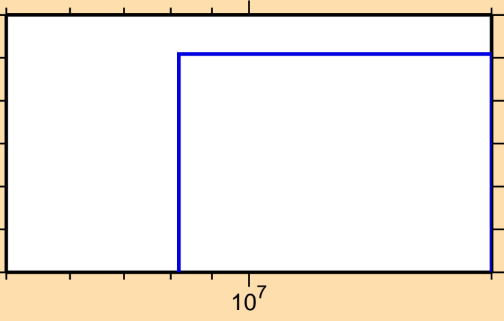
\sigma vs. E for ^{158}\text{Dy}(n,t)
