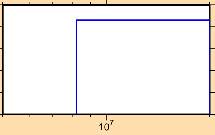
\sigma vs. E for ^{158}\text{Dy}(n,3n)
