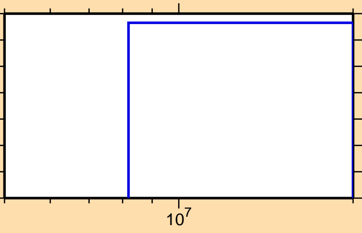
\sigma vs. E for ^{158}\text{Dy}(n,p\alpha)
