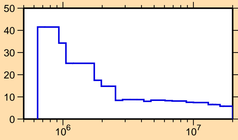
\Delta\sigma/\sigma vs. E for ^{159}\text{Dy}(n,n\text{onel.})
