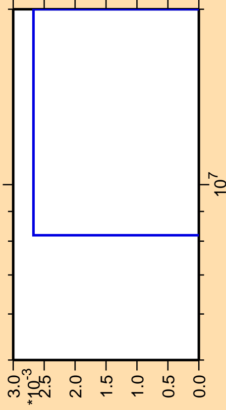
\Delta\sigma/\sigma vs. E for ^{159}\text{Dy} (mt 34)
