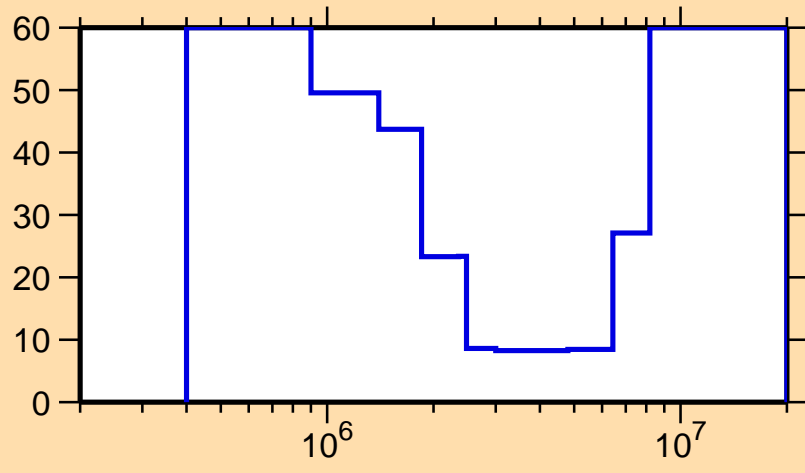
\Delta\sigma/\sigma vs. E for ^{159}\text{Dy}(n,n\text{cont.})
