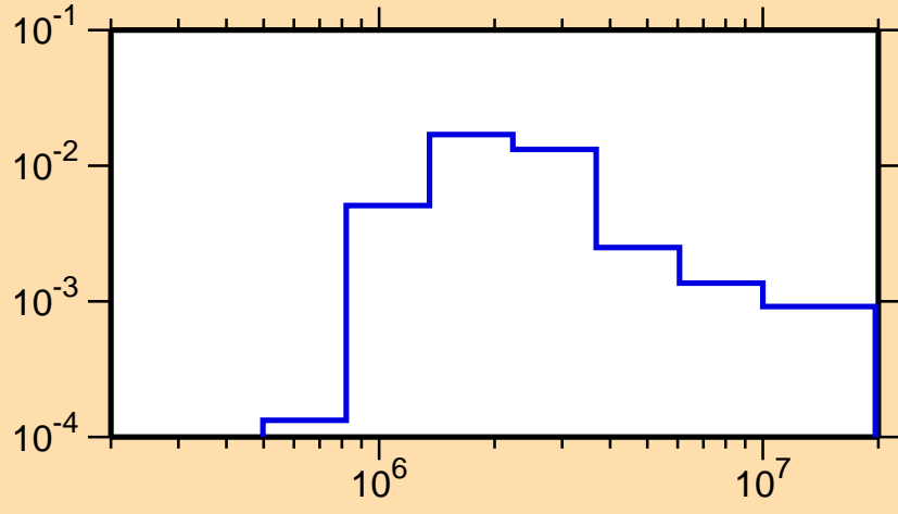
\sigma vs. E for ^{160}\text{Dy}(n,n_3)
