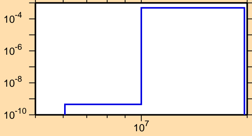
\sigma vs. E for ^{160}\text{Dy}(n,d)
