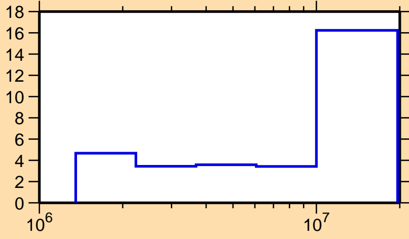
\Delta\sigma/\sigma vs. E for ^{160}\text{Dy}(n,n\text{cont.})
