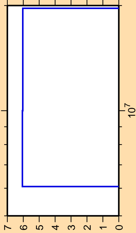
\Delta\sigma/\sigma vs. E for ^{160}\text{Dy}(n,2n)
