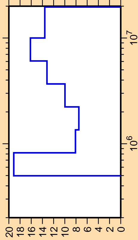
\Delta\sigma/\sigma vs. E for ^{160}\text{Dy}(n,n_3)
