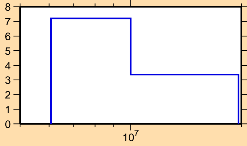
\Delta\sigma/\sigma vs. E for ^{160}\text{Dy}(n,\text{el.})
