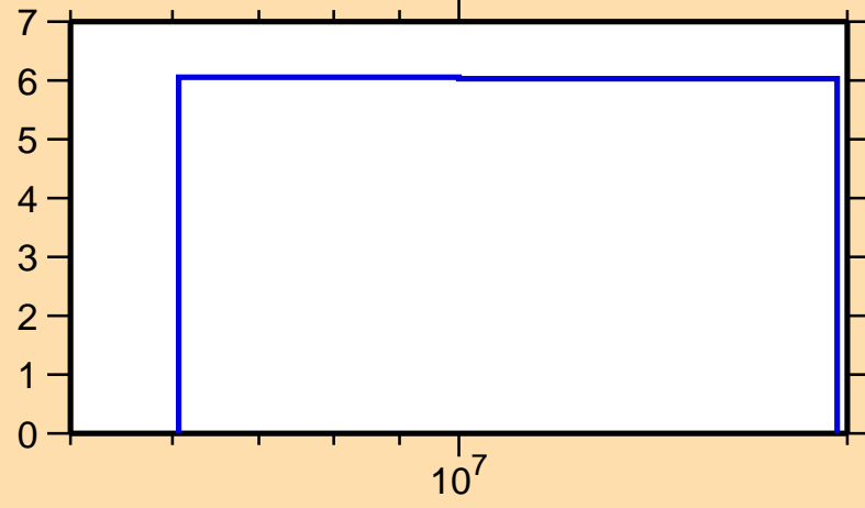
\Delta\sigma/\sigma vs. E for ^{160}\text{Dy}(n,2n)
