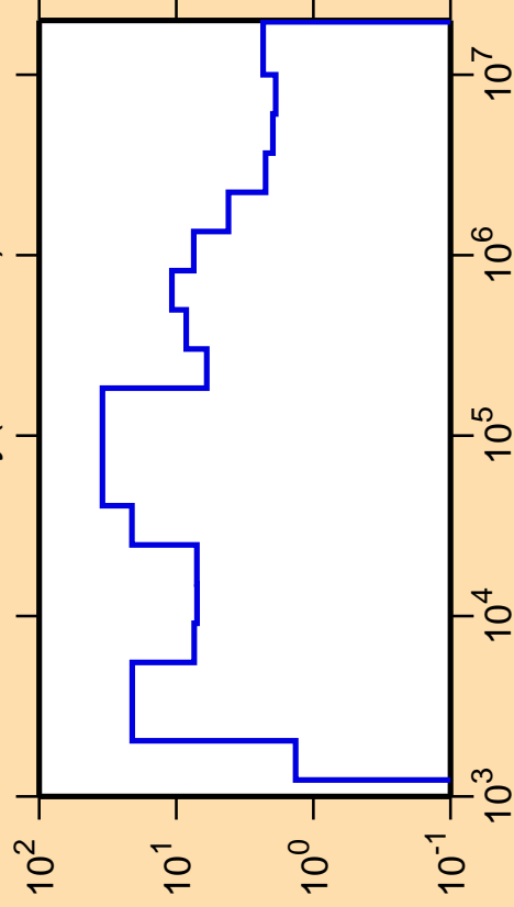
\Delta\sigma/\sigma vs. E for ^{160}\text{Dy}(n,\text{nonel.})
