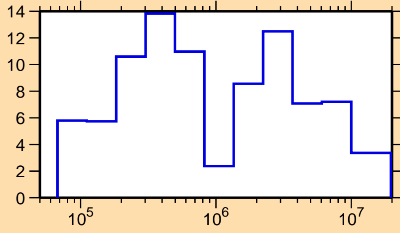
\Delta\sigma/\sigma vs. E for ^{160}\text{Dy}(n,\text{el.})
