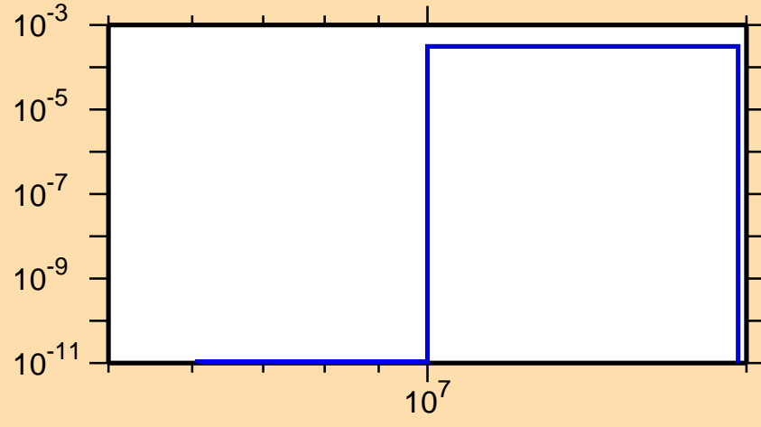
\sigma vs. E for ^{160}\text{Dy}(n,np)
