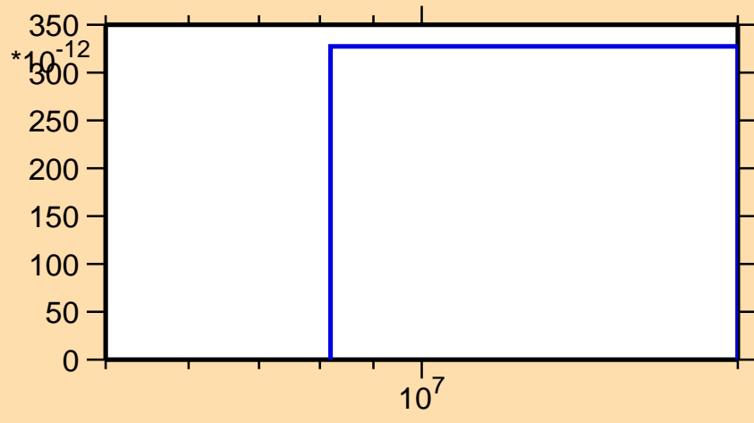
\sigma vs. E for ^{160}\text{Dy}(n,nd)
