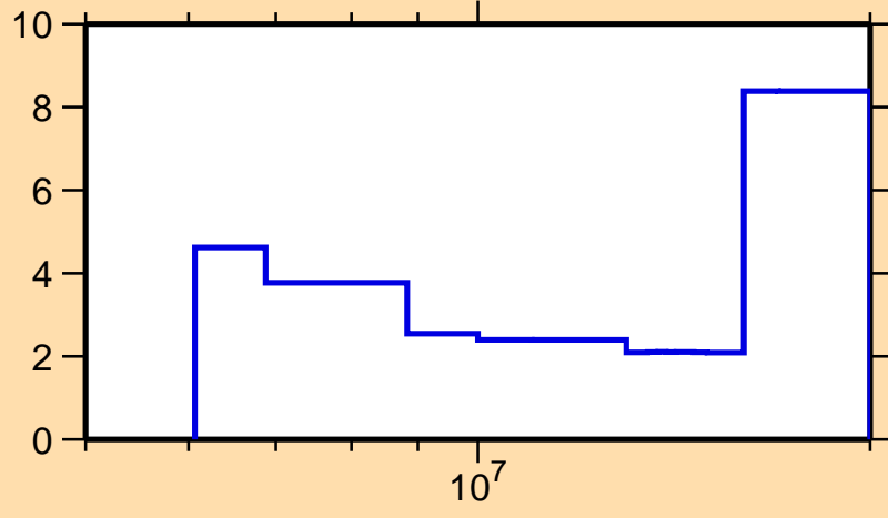
\Delta\sigma/\sigma vs. E for ^{161}\text{Dy}(n,2n)
