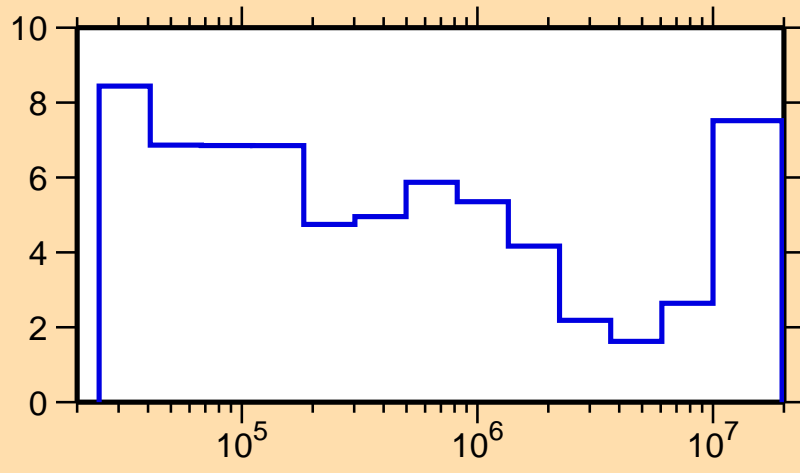
\Delta\sigma/\sigma vs. E for ^{161}\text{Dy}(n,\text{inel.})
