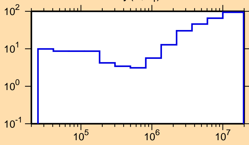
\Delta\sigma/\sigma vs. E for ^{161}\text{Dy}(n,n_1)
