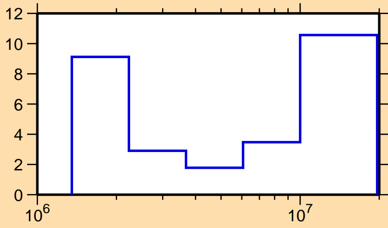
\Delta\sigma/\sigma vs. E for ^{161}\text{Dy}(n,n\text{cont.})
