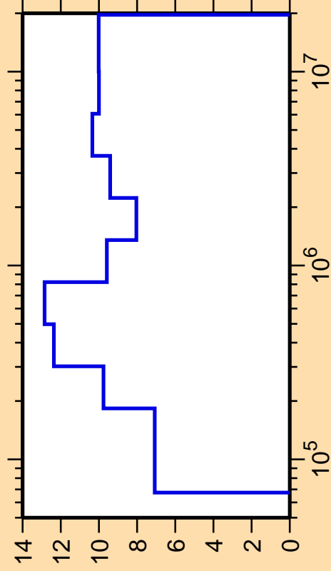
\Delta\sigma/\sigma vs. E for ^{161}\text{Dy}(n,n_4)
