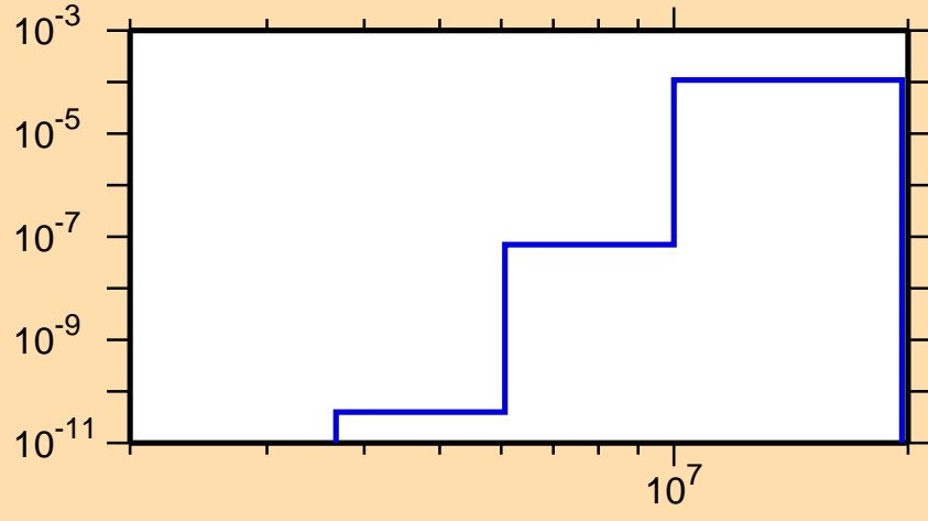
\sigma vs. E for ^{161}\text{Dy}(n,n\alpha)
