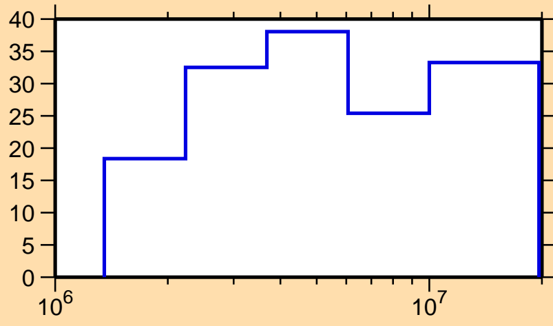
\Delta\sigma/\sigma vs. E for ^{161}\text{Dy}(n,\gamma)
