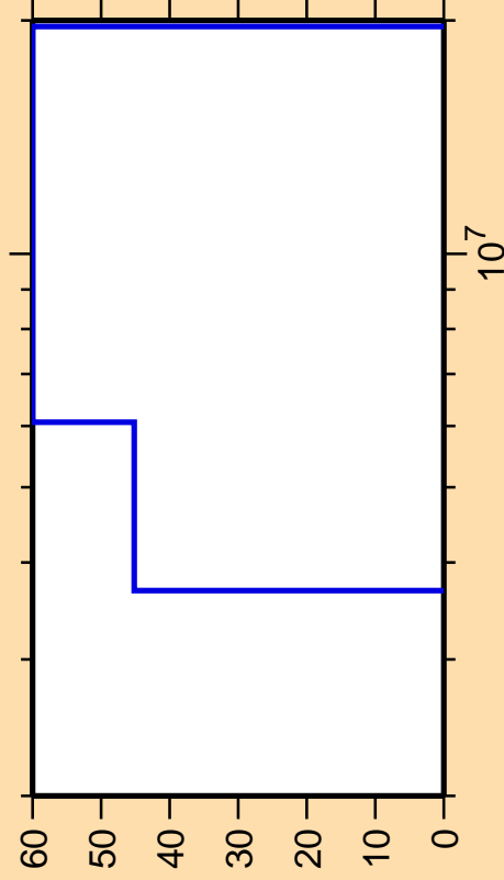
\Delta\sigma/\sigma vs. E for ^{161}\text{Dy}(n,n\alpha)
