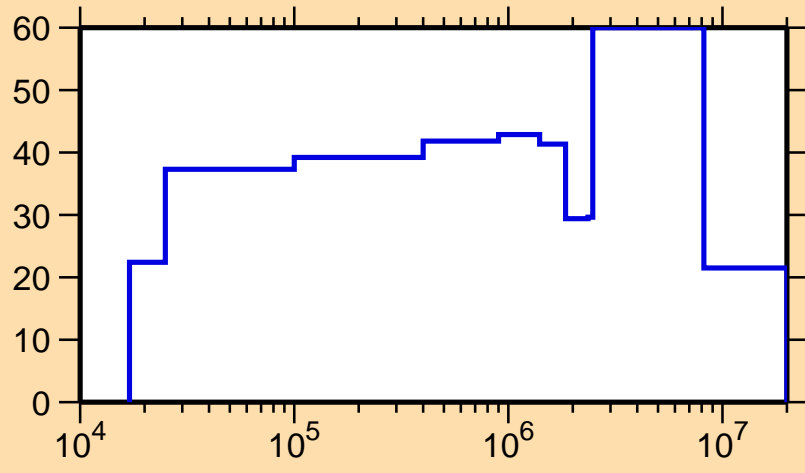
\Delta\sigma/\sigma vs. E for ^{162}\text{Dy}(n,\gamma)
