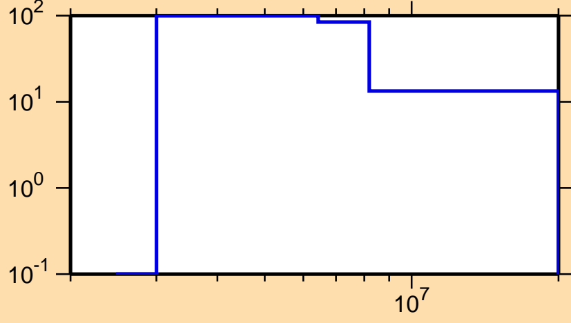
\Delta\sigma/\sigma vs. E for ^{162}\text{Dy}(n,p)
