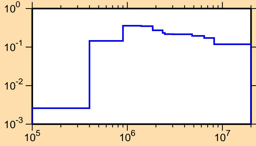
\sigma vs. E for ^{162}\text{Dy}(n,n_2)
