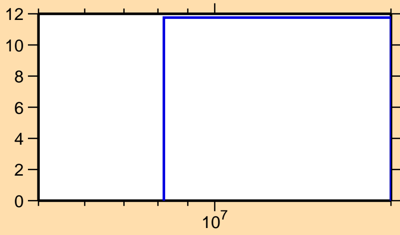
\Delta\sigma/\sigma vs. E for ^{162}\text{Dy}(n,2n)
