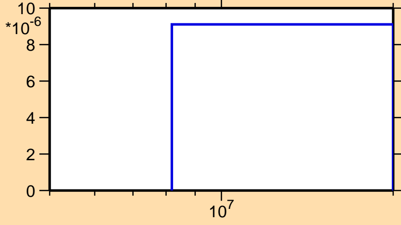
\sigma vs. E for ^{162}\text{Dy}(n,t)
