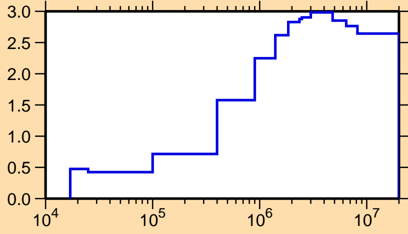
\sigma vs. E for ^{162}\text{Dy}(n,\text{nonel.})
