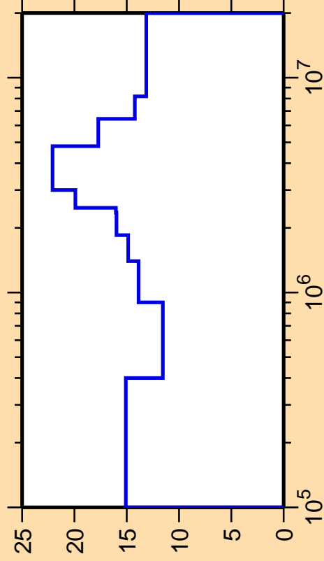
\Delta\sigma/\sigma vs. E for ^{162}\text{Dy}(n,n_2)
