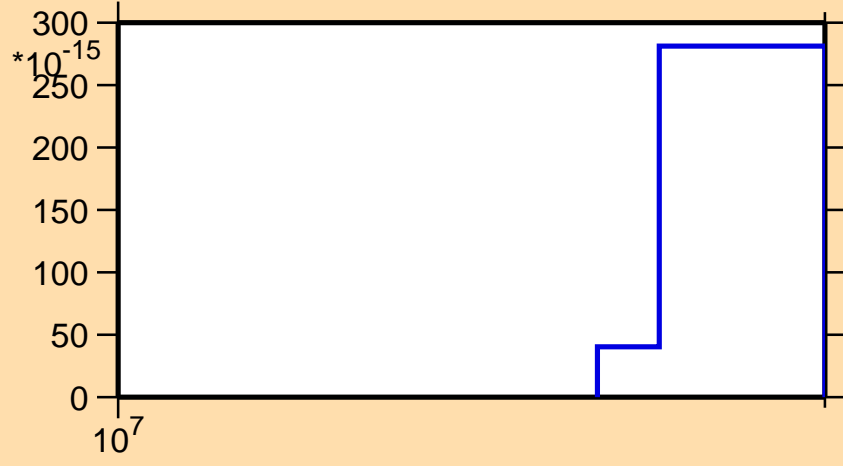
\sigma vs. E for ^{163}\text{Dy}(n,p\alpha)
