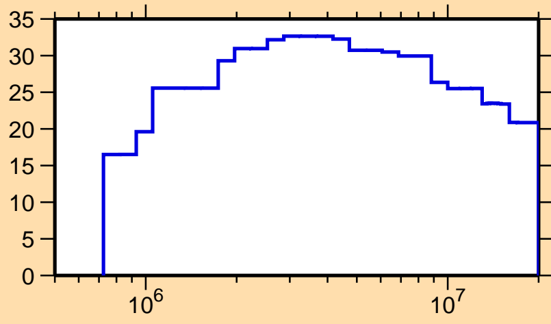
\Delta\sigma/\sigma vs. E for ^{163}\text{Dy}(n, n_1)
