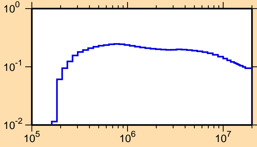
\sigma vs. E for ^{163}\text{Dy}(n,n_2)
