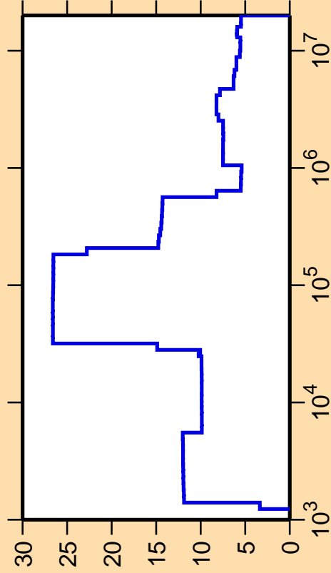
\Delta\sigma/\sigma vs. E for ^{163}\text{Dy}(n,\text{nonel.})
