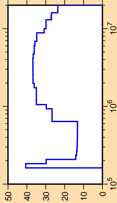
\Delta\sigma/\sigma vs. E for ^{163}\text{Dy}(n,n_2)
