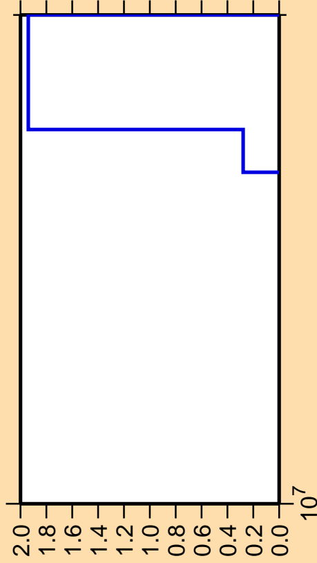
\Delta\sigma/\sigma vs. E for ^{163}\text{Dy}(n,p\alpha)
