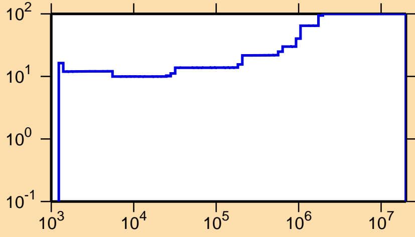
\Delta\sigma/\sigma vs. E for ^{163}\text{Dy}(n,\gamma)
