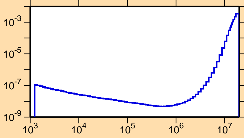
\sigma vs. E for ^{163}\text{Dy}(n,\alpha)
