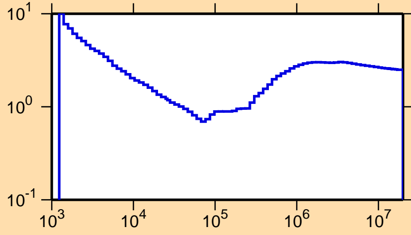
\sigma vs. E for ^{163}\text{Dy}(n,\text{nonel.})
