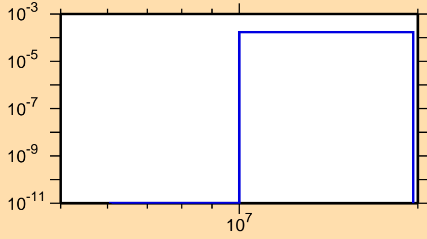
\sigma vs. E for ^{163}\text{Dy}(n,d)
