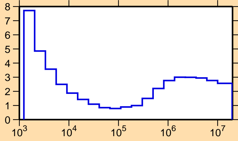
\sigma vs. E for ^{163}\text{Dy}(n,\text{nonel.})
