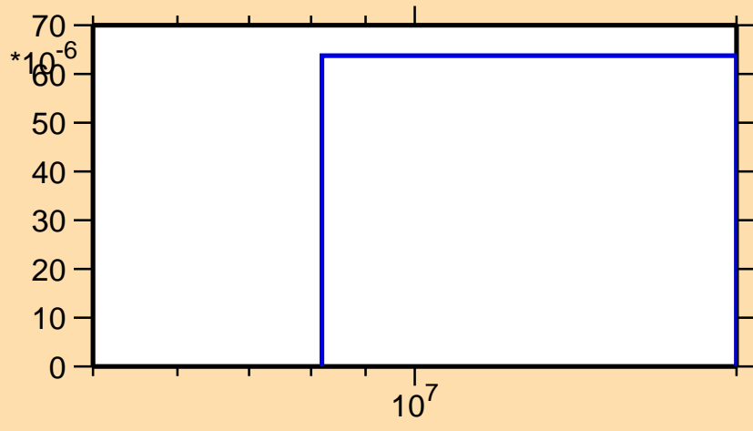
\sigma vs. E for ^{163}\text{Dy}(n,np)
