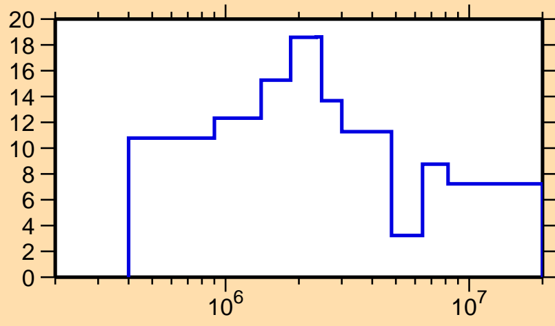
\Delta\sigma/\sigma vs. E for ^{163}\text{Dy}(n,el.)
