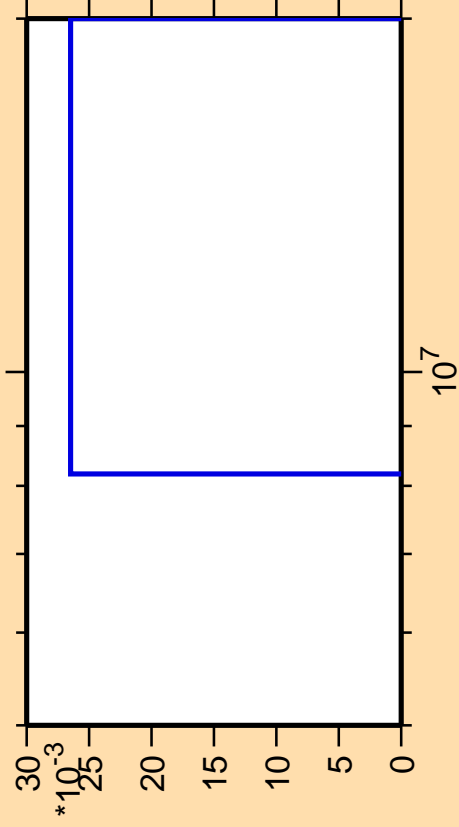
\Delta\sigma/\sigma vs. E for ^{163}\text{Dy}(n,p\alpha)
