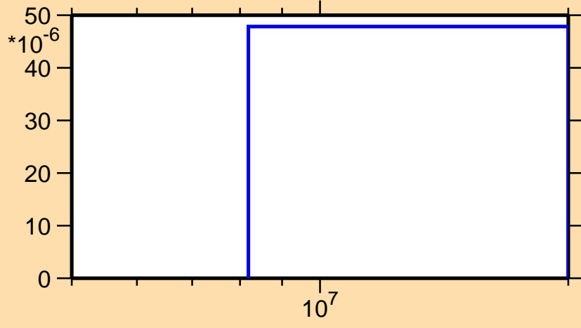
\sigma vs. E for ^{163}\text{Dy}(n,t)
