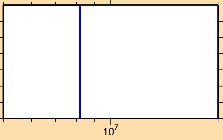
\sigma vs. E for ^{163}\text{Dy}(n,\text{He3})
