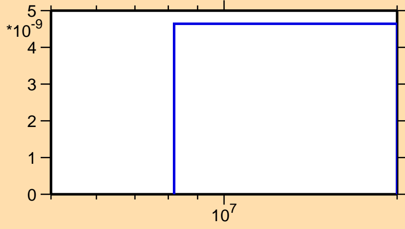
\sigma vs. E for ^{163}\text{Dy}(n,nd)
