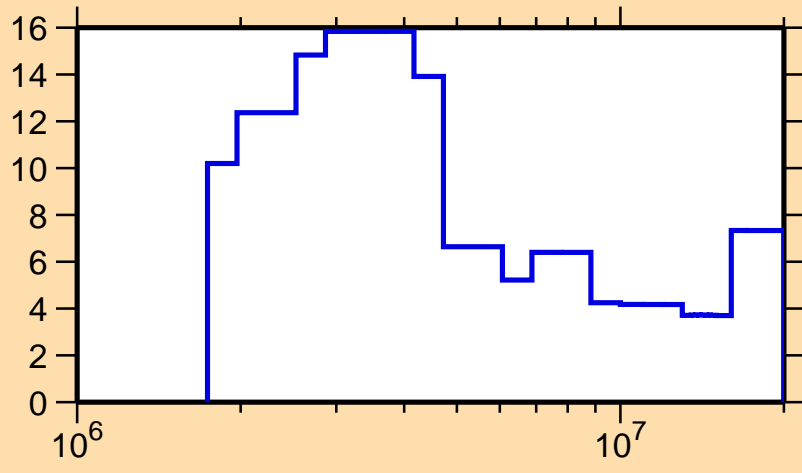
\Delta\sigma/\sigma vs. E for ^{164}\text{Dy}(n,el.)
