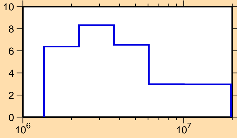
\Delta\sigma/\sigma vs. E for ^{164}\text{Dy}(n,tot.)
