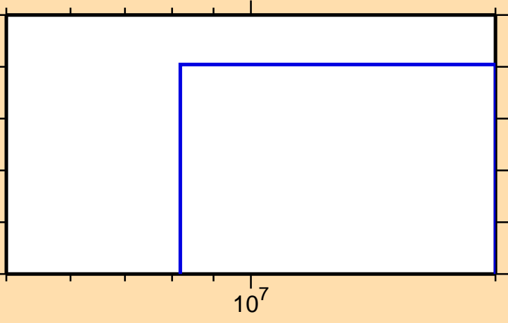
\sigma vs. E for ^{164}\text{Dy}(n,np)
