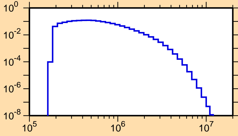
\sigma vs. E for ^{165}\text{Dy}(n,n_4)
