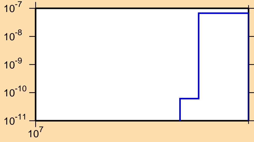
\sigma vs. E for ^{165}\text{Dy}(n,2np)
