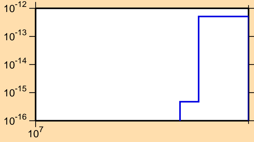
\sigma vs. E for ^{165}\text{Dy}(n,\text{He3})
