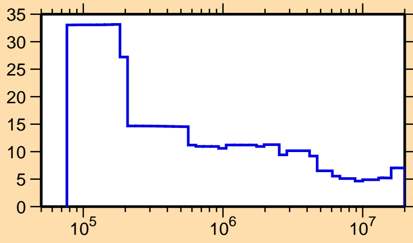
\Delta\sigma/\sigma vs. E for ^{165}\text{Dy}(n,\text{tot.})
