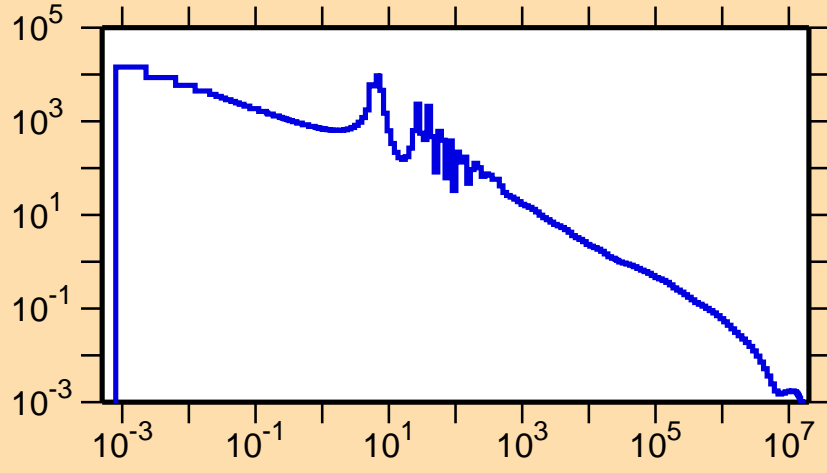
\sigma vs. E for ^{165}\text{Dy}(n,\gamma)
