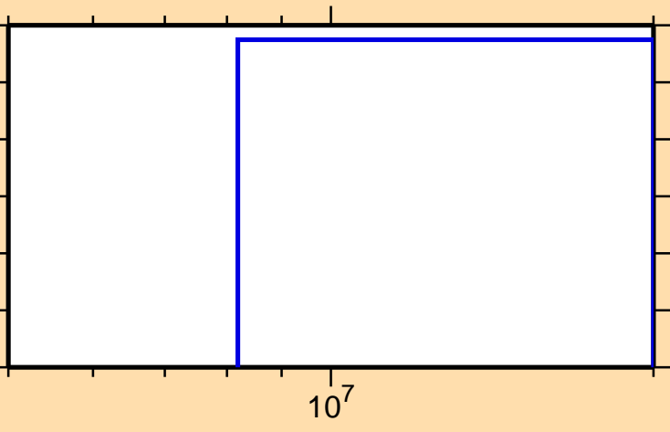
\sigma vs. E for ^{165}\text{Dy}(n,d)
