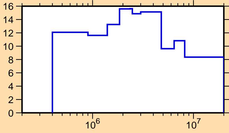
\Delta\sigma/\sigma vs. E for ^{165}\text{Dy}(n,el.)
