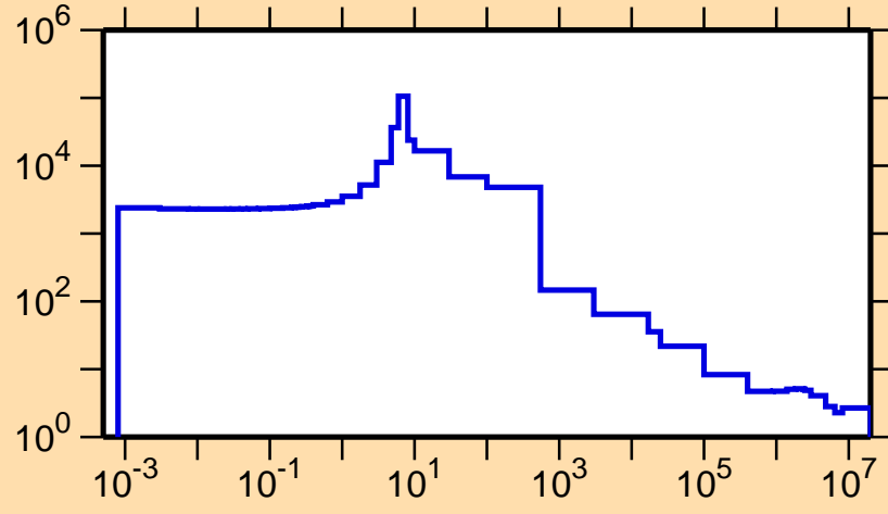
\sigma vs. E for ^{165}\text{Dy}(n,\text{el.})
