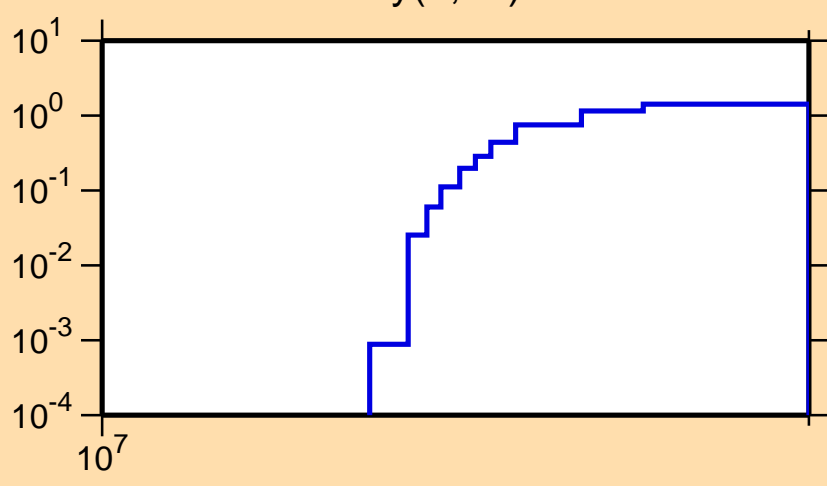
\sigma vs. E for ^{165}\text{Dy}(n,3n)
