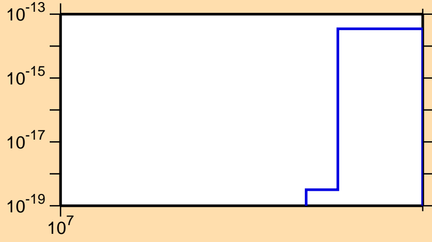
\sigma vs. E for ^{165}\text{Dy}(n,3n\alpha)
