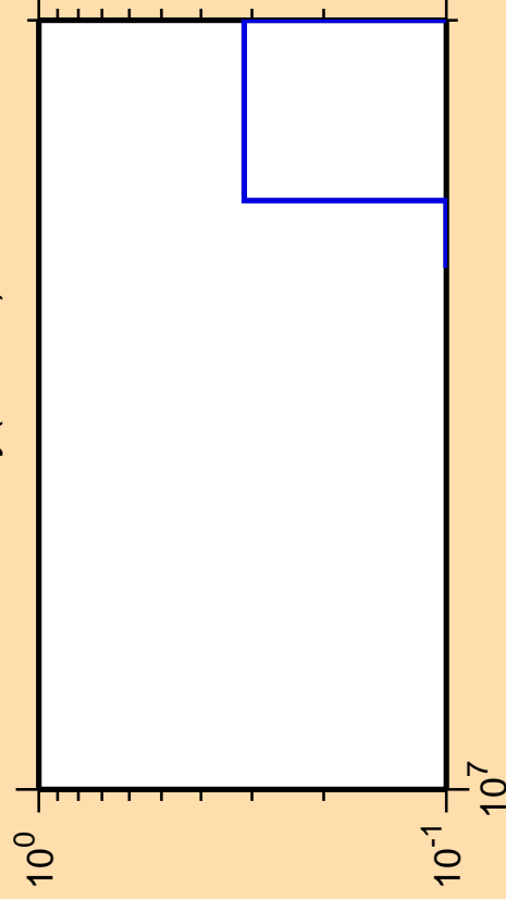
\Delta\sigma/\sigma vs. E for ^{165}\text{Dy}(n,3n\alpha)
