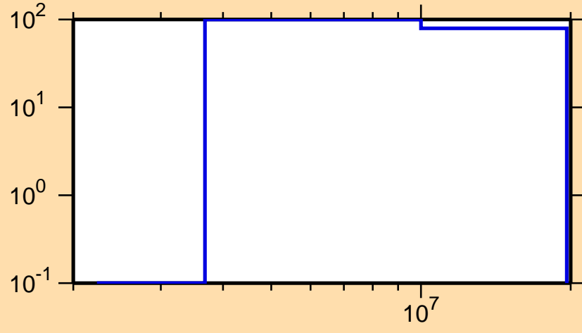
\Delta\sigma/\sigma vs. E for ^{165}\text{Dy}(n,p)
