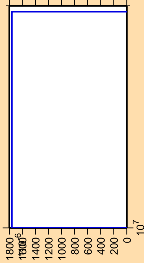
\Delta\sigma/\sigma vs. E for ^{165}\text{Dy}(n,3n\alpha)
