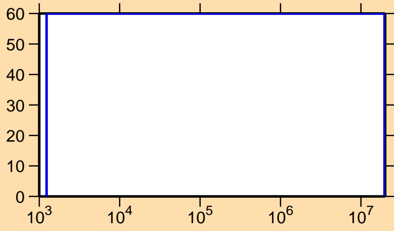
\Delta\sigma/\sigma vs. E for ^{165}\text{Dy}(n,\gamma)
