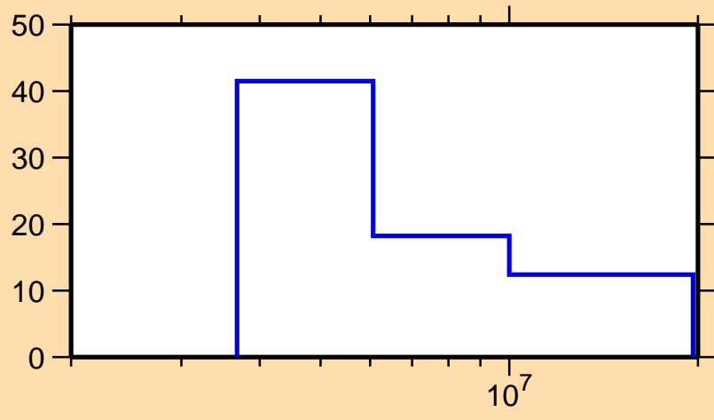
\Delta\sigma/\sigma vs. E for ^{165}\text{Dy}(n,2n)
