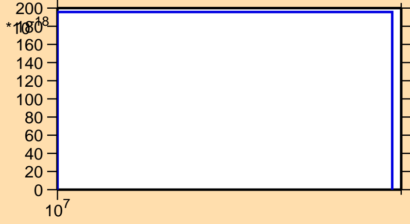
\sigma vs. E for ^{165}\text{Dy}(n,3n\alpha)
