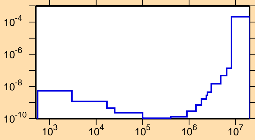
\sigma vs. E for ^{165}\text{Dy}(n,\alpha)
