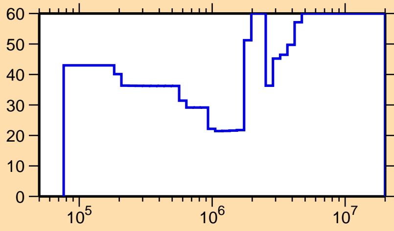
\Delta\sigma/\sigma vs. E for ^{166}\text{Dy}(n,n_1)
