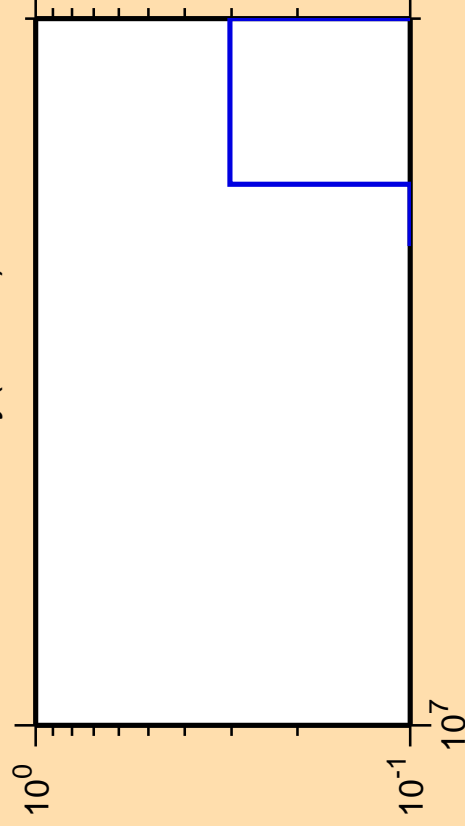
\Delta\sigma/\sigma vs. E for ^{166}\text{Dy}(n,3n\alpha)
