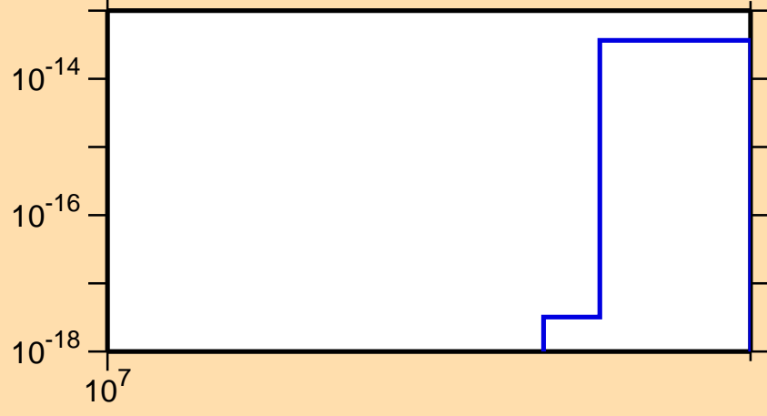
\sigma vs. E for ^{166}\text{Dy}(n,3n\alpha)
