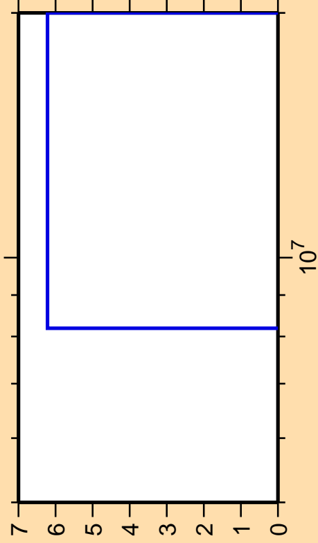
\Delta\sigma/\sigma vs. E for ^{166}\text{Dy}(n,2np)
