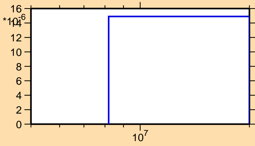
\sigma vs. E for ^{166}\text{Dy}(n,np)
