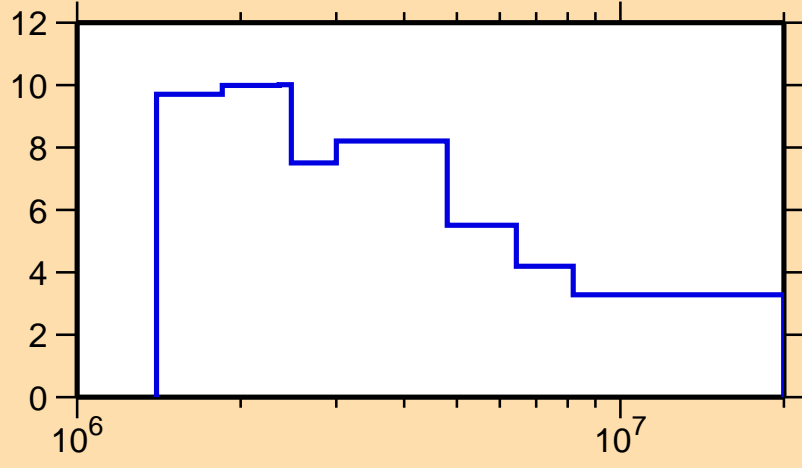
\Delta\sigma/\sigma vs. E for ^{166}\text{Dy}(n,\text{tot.})
