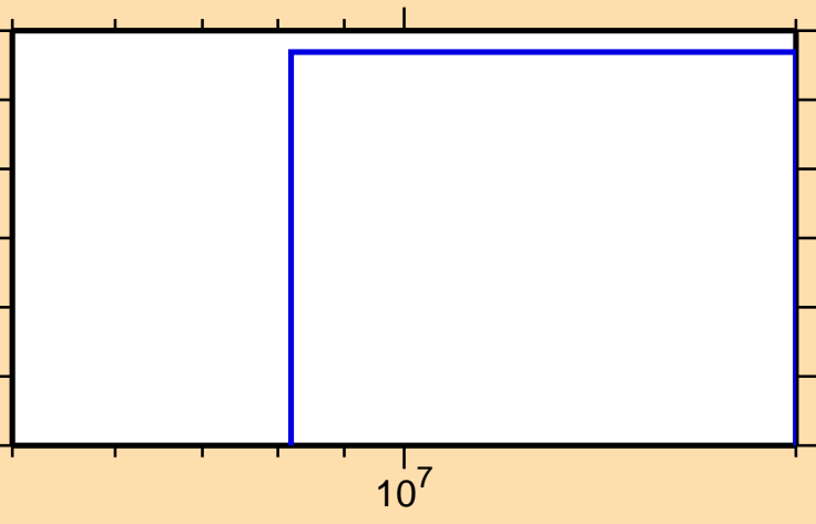
\sigma vs. E for ^{166}\text{Dy}(n,d)
