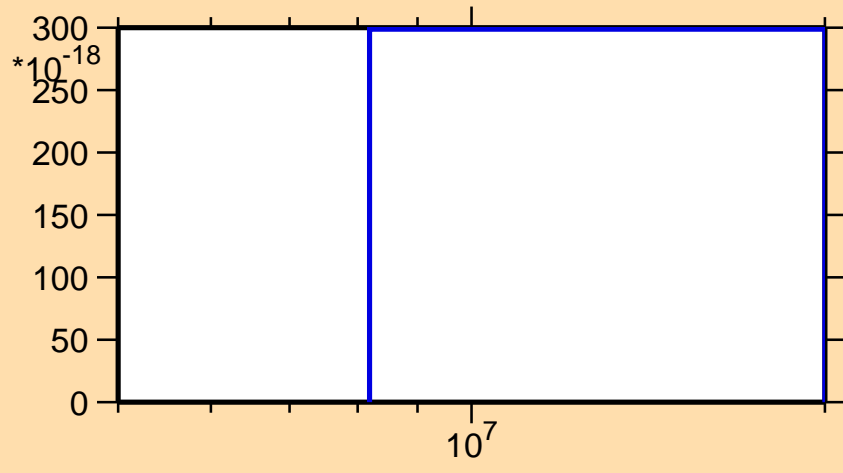
\sigma vs. E for ^{166}\text{Dy}(n,3n\alpha)
