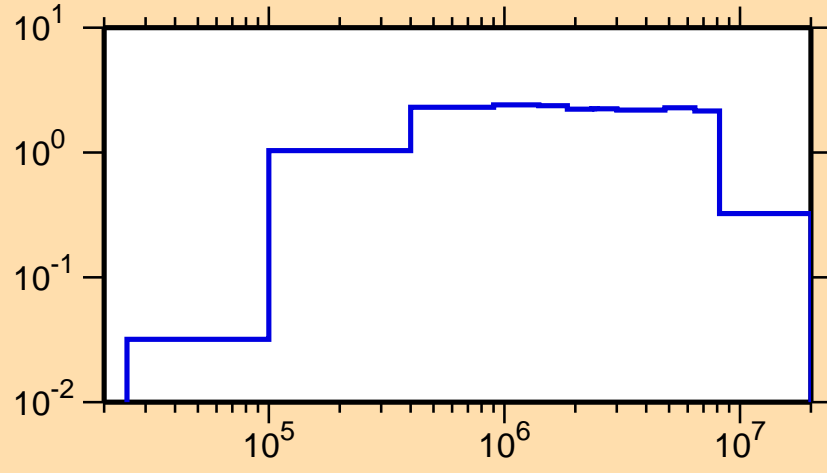
\sigma vs. E for ^{166}\text{Dy}(n,\text{inel.})
