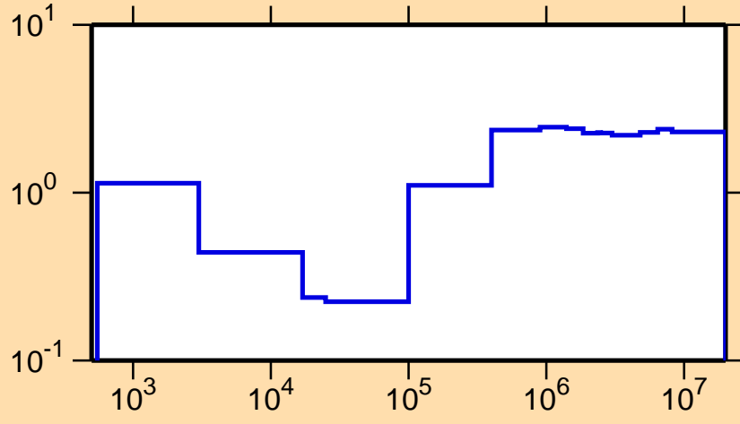
\sigma vs. E for ^{166}\text{Dy}(n,\text{nonel.})
