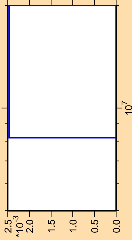
\Delta\sigma/\sigma vs. E for ^{166}\text{Dy}(n,3n\alpha)
