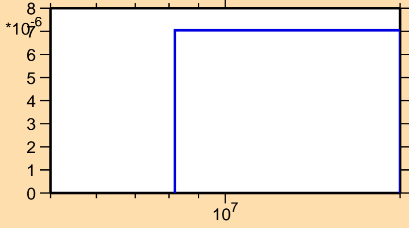
\sigma vs. E for ^{166}\text{Dy}(n,t)
