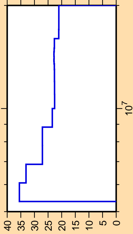
\Delta\sigma/\sigma vs. E for ^{167}\text{Dy}(n,n_1)
