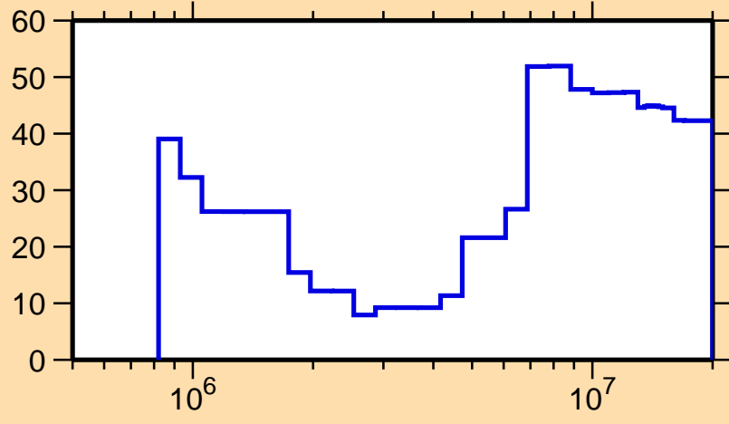
\Delta\sigma/\sigma vs. E for ^{167}\text{Dy}(n,n\text{cont.})
