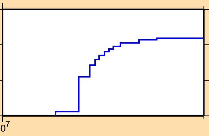
\sigma vs. E for ^{167}\text{Dy}(n,3n)
