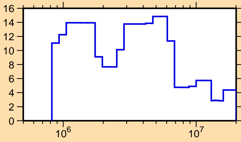
\Delta\sigma/\sigma vs. E for ^{167}\text{Dy}(n,el.)
