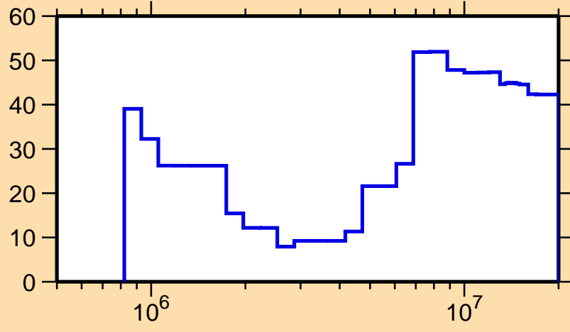
\Delta\sigma/\sigma vs. E for ^{167}\text{Dy}(n,n\text{cont.})
