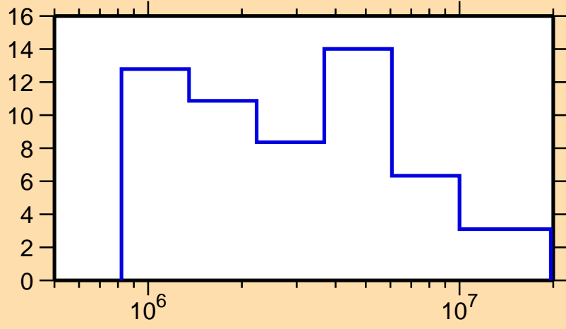
\Delta\sigma/\sigma vs. E for ^{167}\text{Dy}(n,el.)
