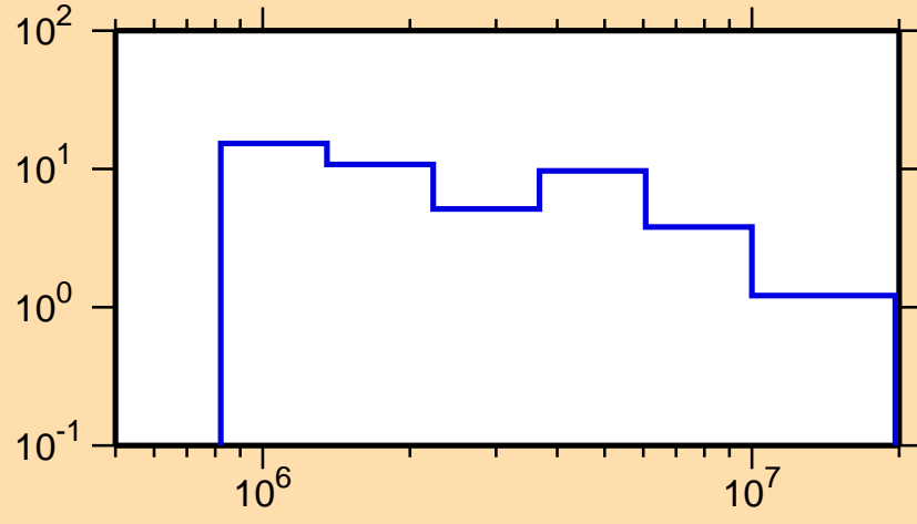
\Delta\sigma/\sigma vs. E for ^{167}\text{Dy}(n, tot.)
