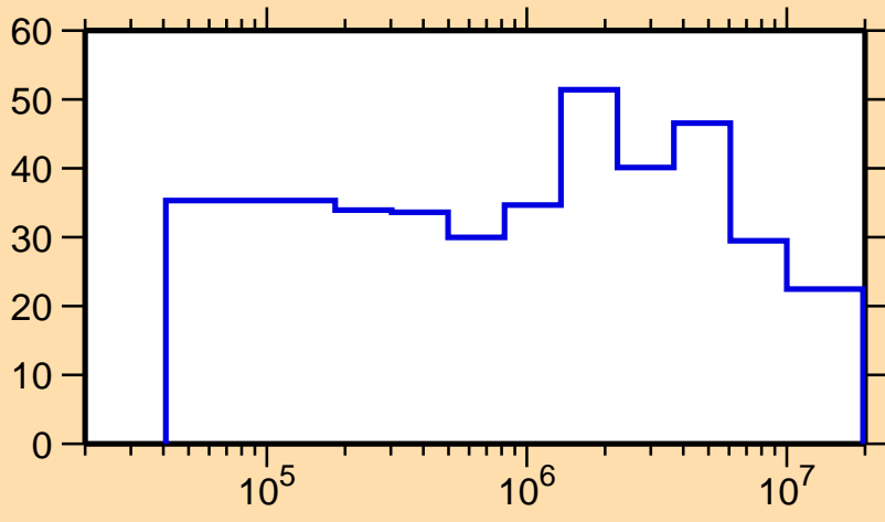
\Delta\sigma/\sigma vs. E for ^{167}\text{Dy}(n,n_1)
