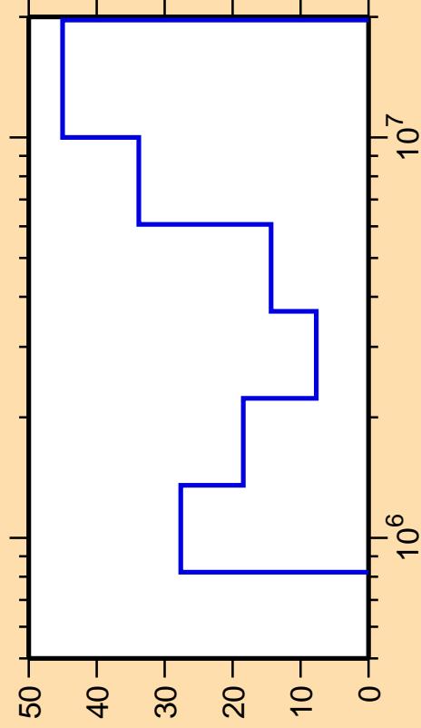
\Delta\sigma/\sigma vs. E for ^{167}\text{Dy}(n, ncont.)
