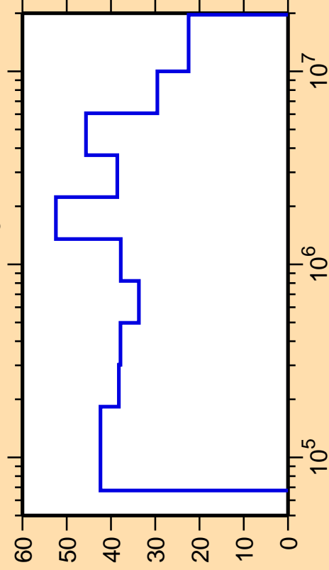
\Delta\sigma/\sigma vs. E for ^{167}\text{Dy}(n,n_3)
