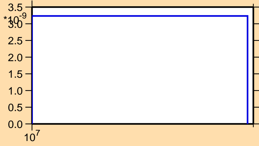
\sigma vs. E for ^{167}\text{Dy}(n,2n\alpha)
