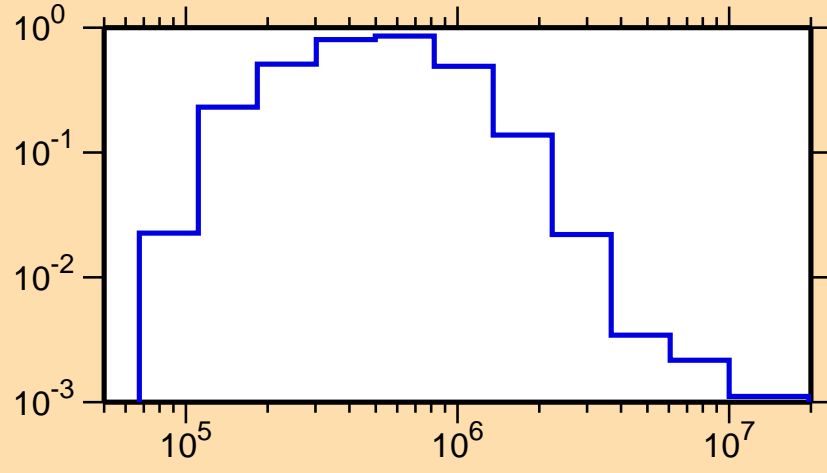
\sigma vs. E for ^{167}\text{Dy}(n,n_3)
