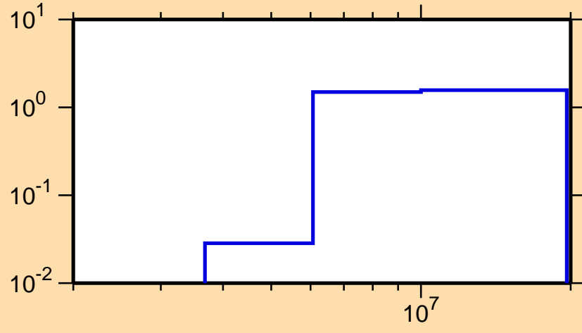
\sigma vs. E for ^{167}\text{Dy}(n,2n)
