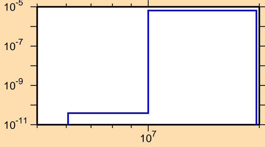
\sigma vs. E for ^{167}\text{Dy}(n,n\alpha)
