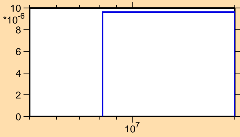
\sigma vs. E for ^{167}\text{Dy}(n,t)
