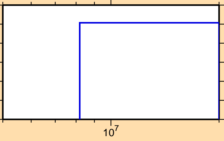
\sigma vs. E for ^{167}\text{Dy}(n,d)
