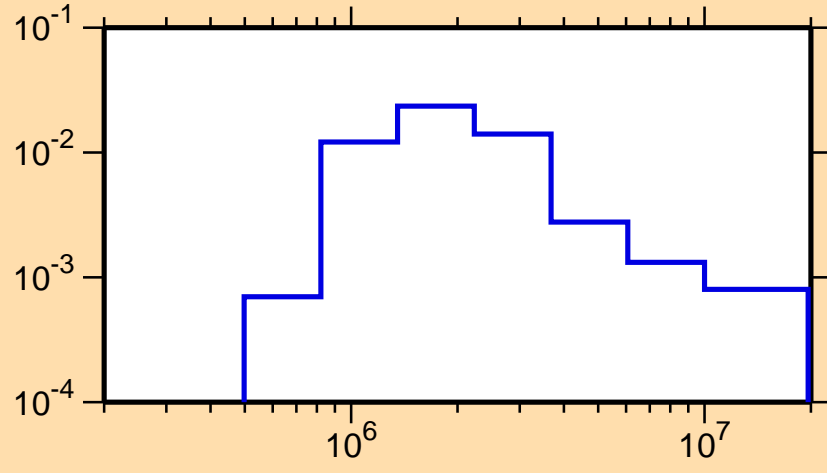
\sigma vs. E for ^{168}\text{Dy}(n,n_3)
