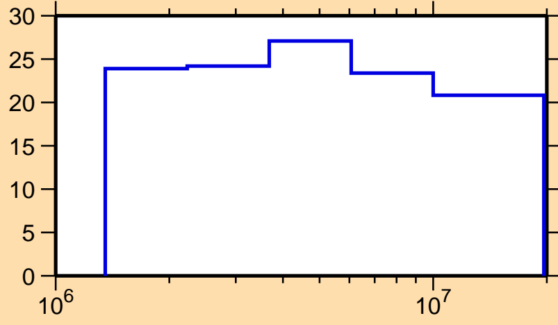
\Delta\sigma/\sigma vs. E for ^{168}\text{Dy}(n,nonel.)
