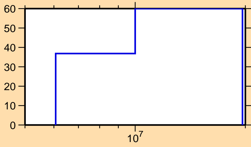
\Delta\sigma/\sigma vs. E for ^{168}\text{Dy}(n,2n)
