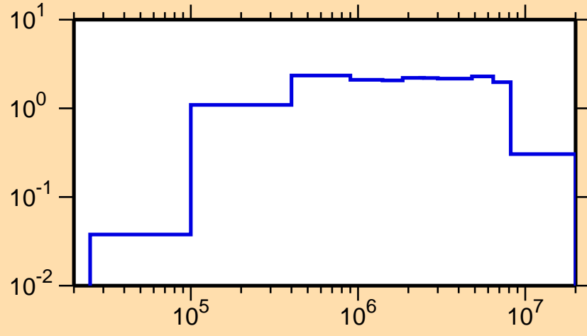
\sigma vs. E for ^{168}\text{Dy}(n,\text{inel.})
