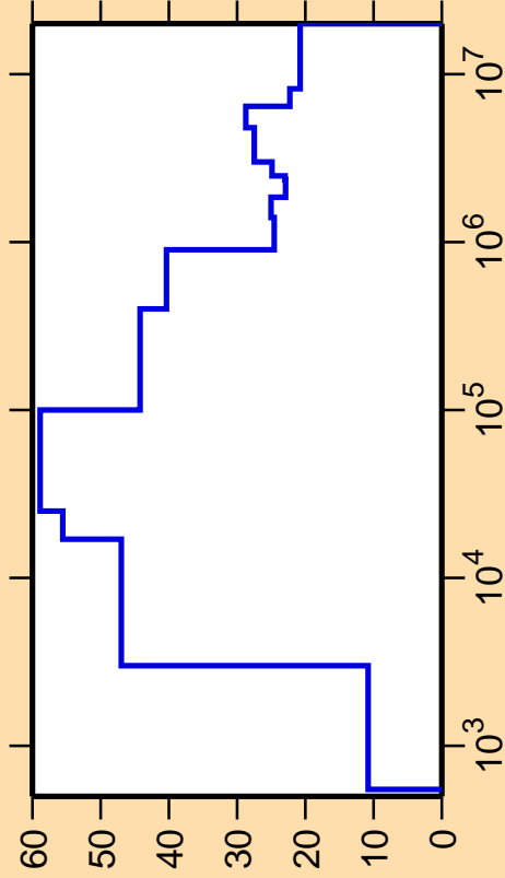
\Delta\sigma/\sigma vs. E for ^{168}\text{Dy}(n,\text{nonel.})
