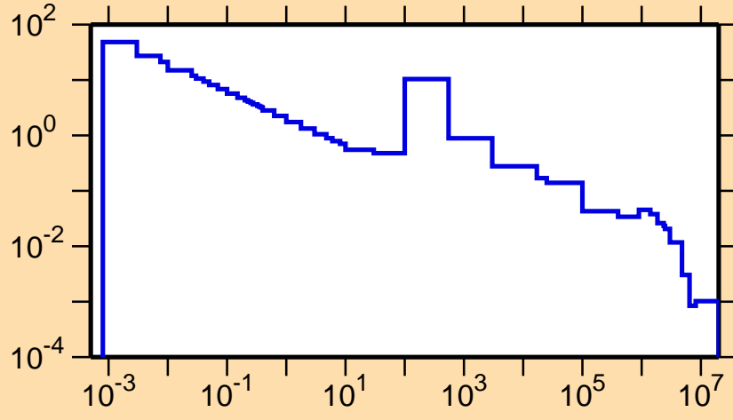
\sigma vs. E for ^{168}\text{Dy}(n,\gamma)
