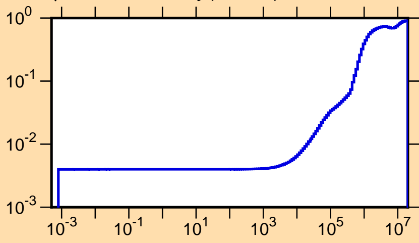
\mu vs. E for ^{169}\text{Dy}(\text{mt251})
