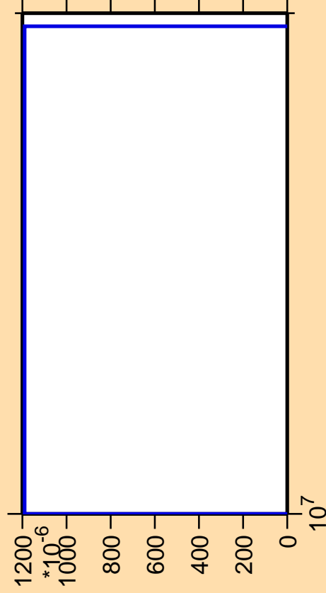
\Delta\sigma/\sigma vs. E for ^{169}\text{Dy}(n,3n\alpha)
