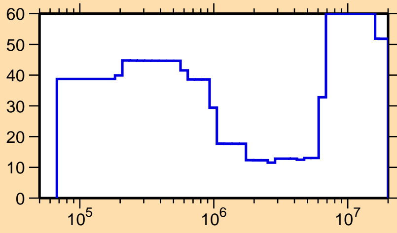
\Delta\sigma/\sigma vs. E for ^{170}\text{Dy}(n,\text{inel.})
