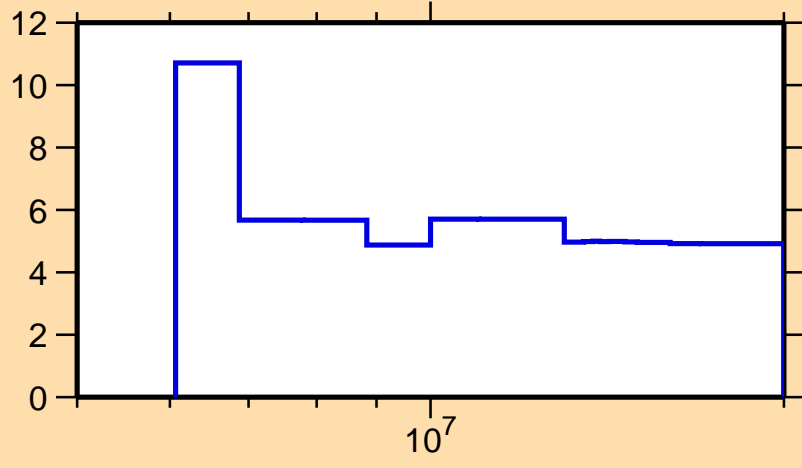
\Delta\sigma/\sigma vs. E for ^{170}\text{Dy}(n,\text{tot.})
