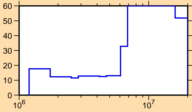
\Delta\sigma/\sigma vs. E for ^{170}\text{Dy}(n,inel.)
