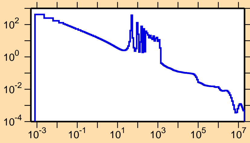
\sigma vs. E for ^{170}\text{Dy}(n,\gamma)
