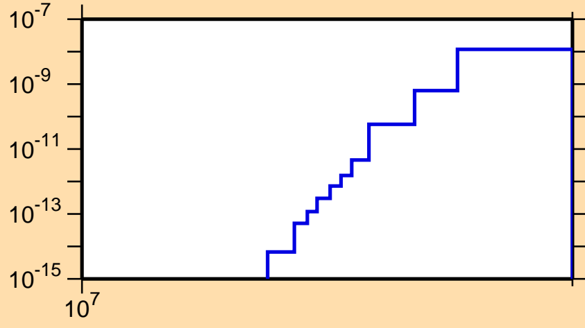
\sigma vs. E for ^{170}\text{Dy}(n,2n\alpha)
