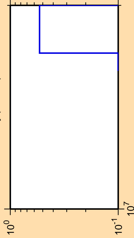
\Delta\sigma/\sigma vs. E for ^{170}\text{Dy}(n,3n\alpha)
