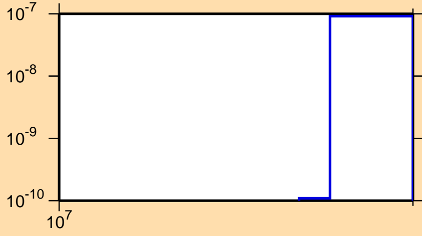
\sigma vs. E for ^{170}\text{Dy}(n,nt)
