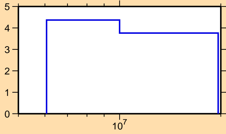
\Delta\sigma/\sigma vs. E for ^{170}\text{Dy}(n,\text{nonel.})
