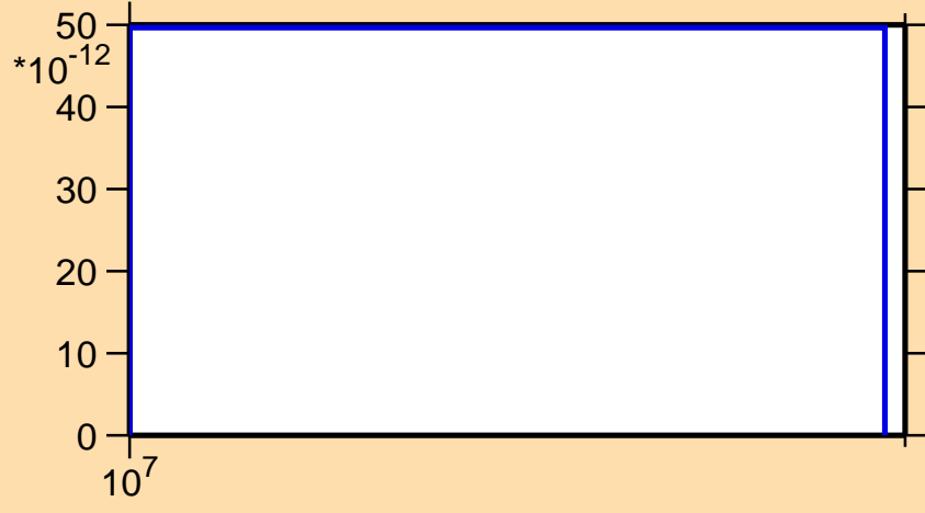
\sigma vs. E for ^{170}\text{Dy}(n,nd)
