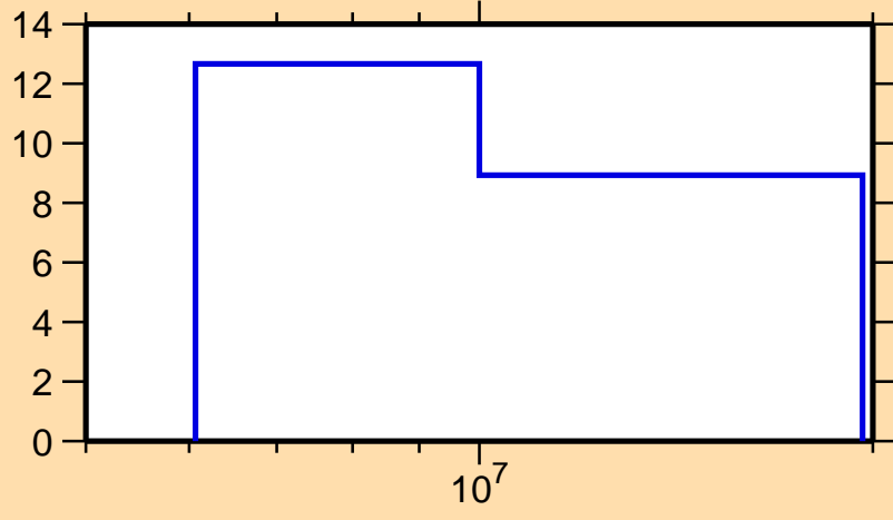
\Delta\sigma/\sigma vs. E for ^{170}\text{Dy}(n,el.)
