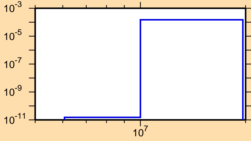
\sigma vs. E for ^{170}\text{Dy}(n,p)
