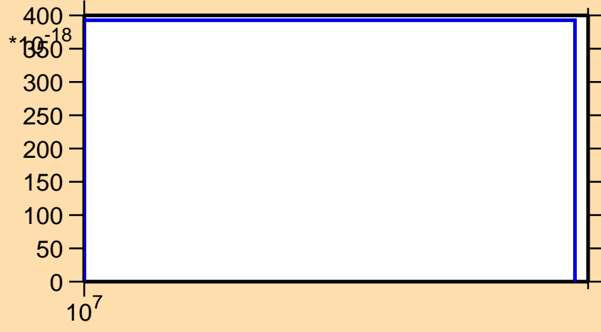
\sigma vs. E for ^{170}\text{Dy}(n,3n\alpha)
