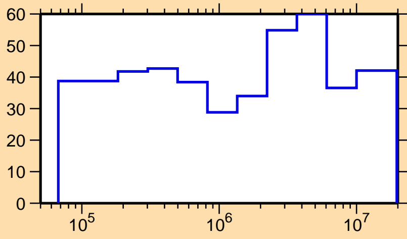
\Delta\sigma/\sigma vs. E for ^{170}\text{Dy}(n,n_1)
