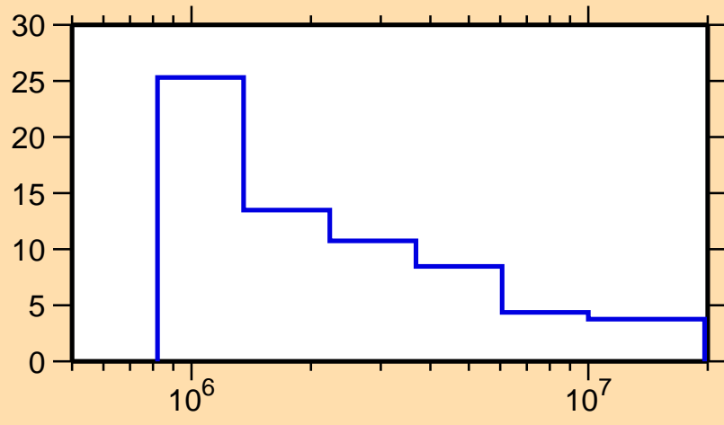
\Delta\sigma/\sigma vs. E for ^{170}\text{Dy}(n,\text{nonel.})
