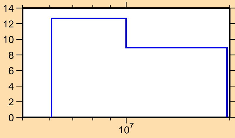
\Delta\sigma/\sigma vs. E for ^{170}\text{Dy}(n,\text{el.})
