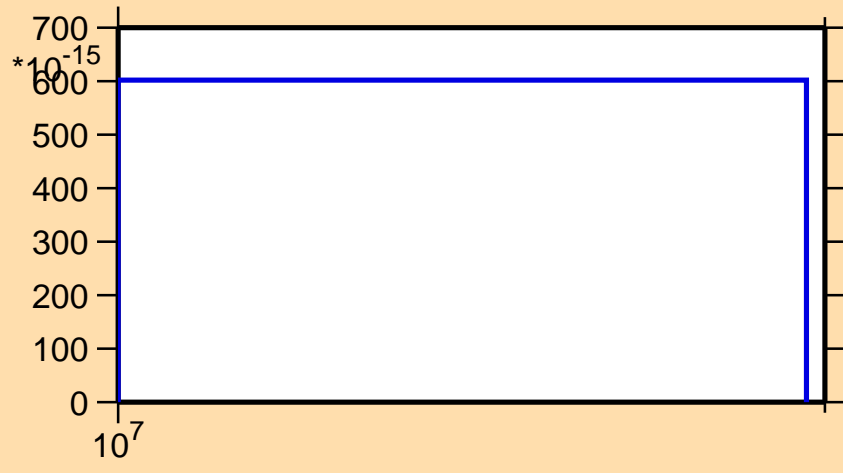
\sigma vs. E for ^{170}\text{Dy}(n,2np)
