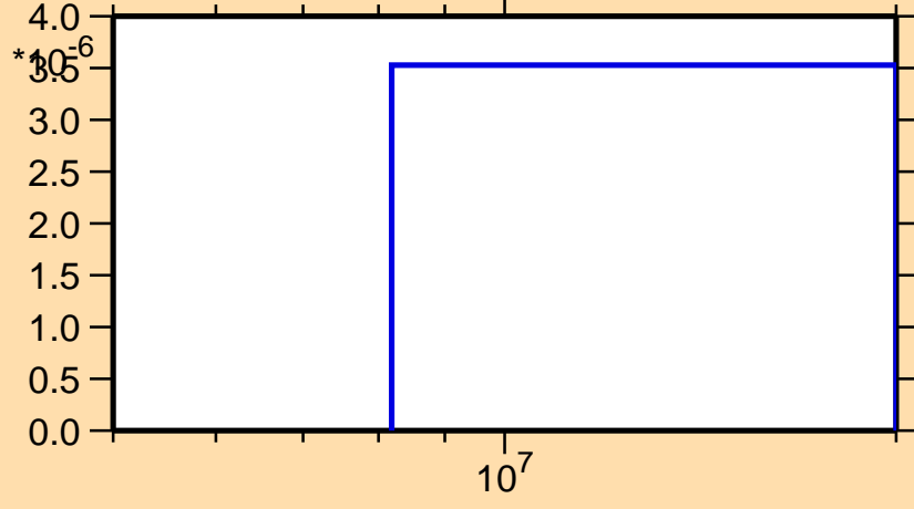
\sigma vs. E for ^{170}\text{Dy}(n,d)
