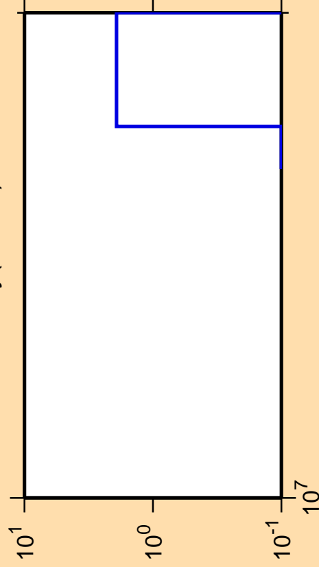
\Delta\sigma/\sigma vs. E for ^{171}\text{Dy}(n,3n\alpha)
