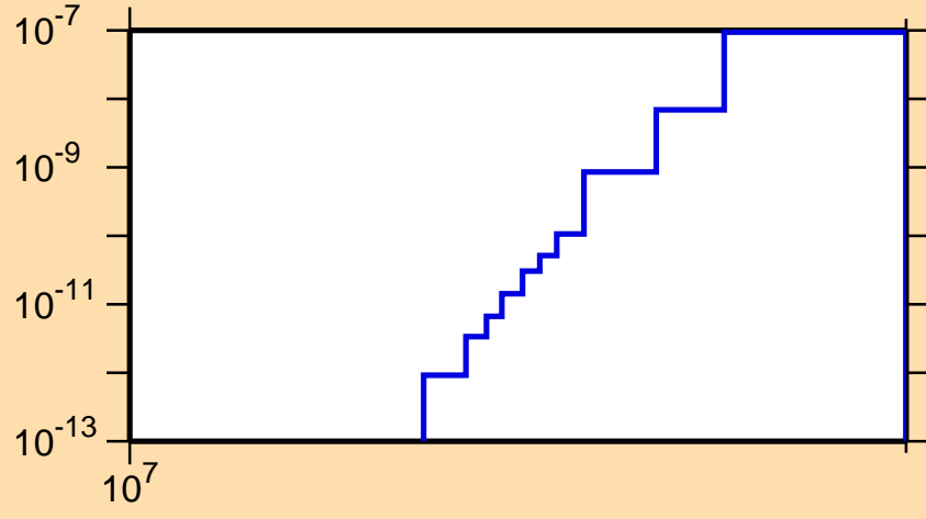
\sigma vs. E for ^{171}\text{Dy}(n,2n\alpha)
