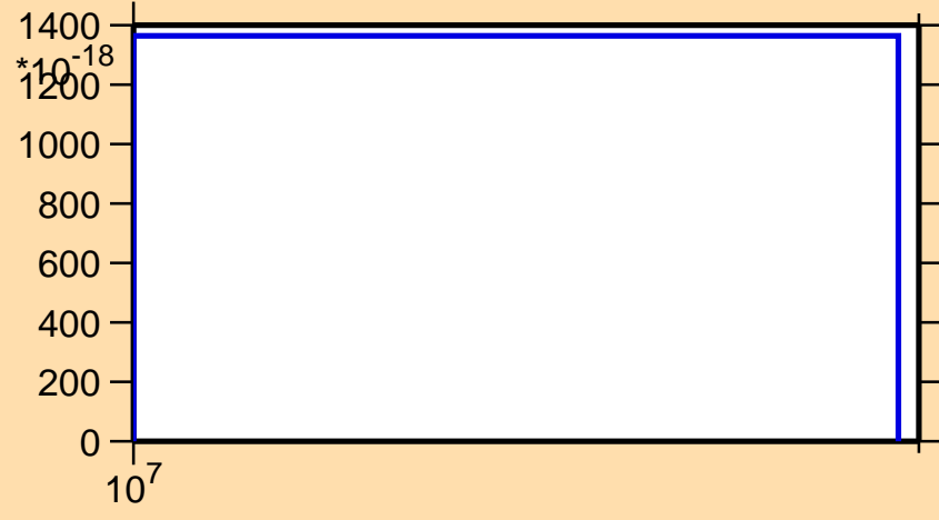
\sigma vs. E for ^{171}\text{Dy}(n,3n\alpha)
