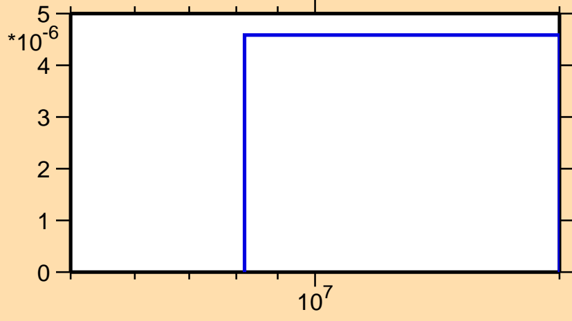
\sigma vs. E for ^{171}\text{Dy}(n,t)
