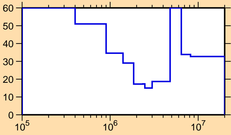
\Delta\sigma/\sigma vs. E for ^{171}\text{Dy}(n,n\text{cont.})
