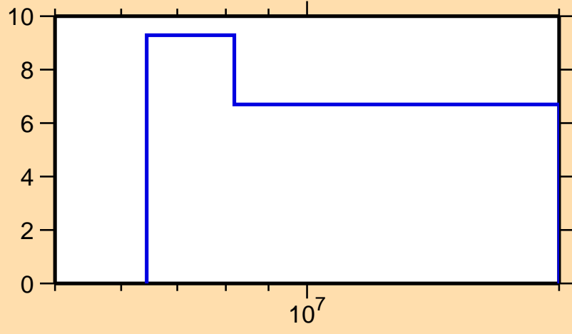
\Delta\sigma/\sigma vs. E for ^{171}\text{Dy}(n,\text{nonel.})
