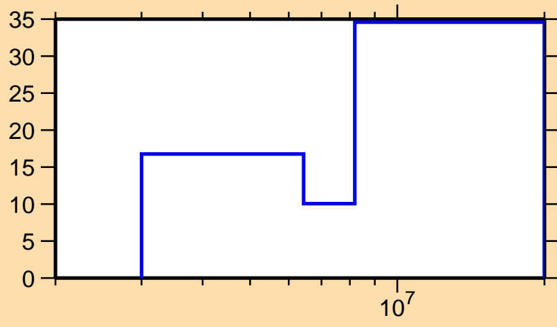
\Delta\sigma/\sigma vs. E for ^{171}\text{Dy}(n,2n)
