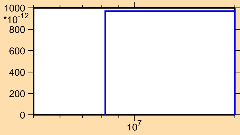
\sigma vs. E for ^{171}\text{Dy}(n,nd)
