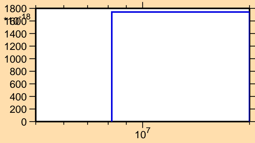
\sigma vs. E for ^{171}\text{Dy}(n,3n\alpha)
