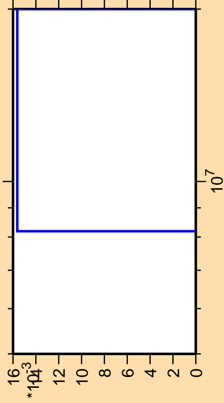
\Delta\sigma/\sigma vs. E for ^{171}\text{Dy}(n,3n\alpha)
