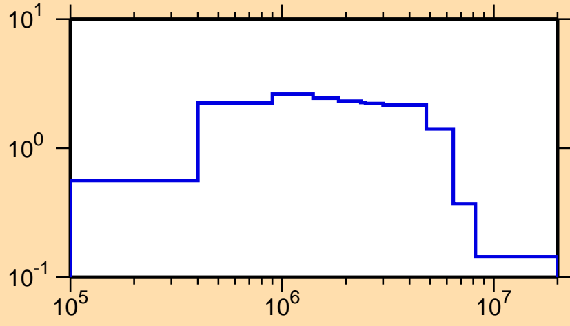
\sigma vs. E for ^{171}\text{Dy}(n,\text{inel.})
