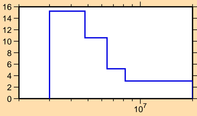
\Delta\sigma/\sigma vs. E for ^{171}\text{Dy}(n,\text{tot.})
