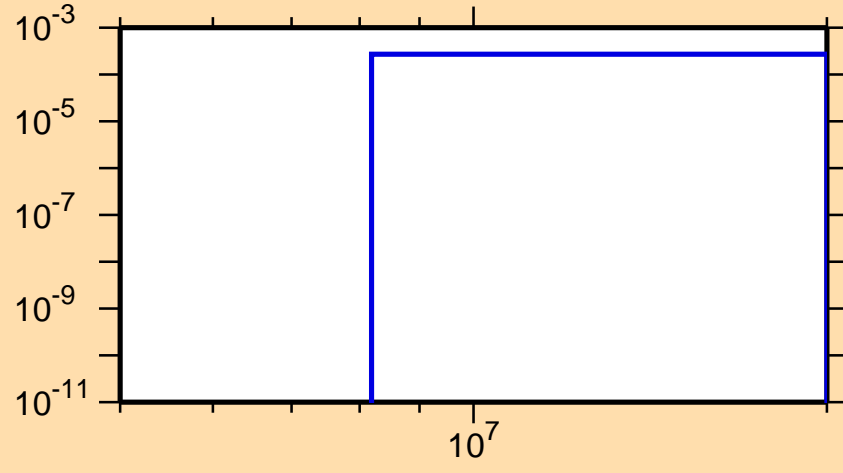
\sigma vs. E for ^{171}\text{Dy}(n,p)
