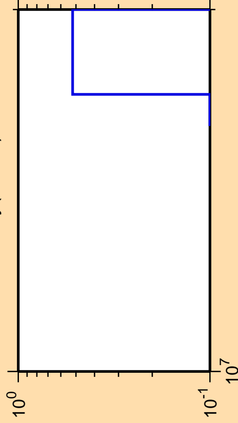
\Delta\sigma/\sigma vs. E for ^{172}\text{Dy}(n,3n\alpha)
