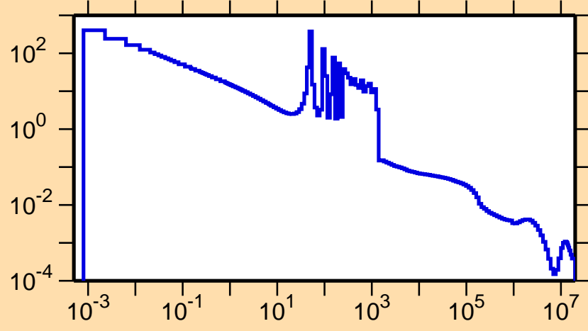
\sigma vs. E for ^{172}\text{Dy}(n,\gamma)
