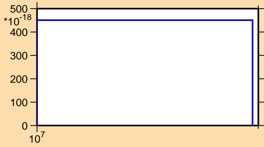
\sigma vs. E for ^{172}\text{Dy}(n,3n\alpha)
