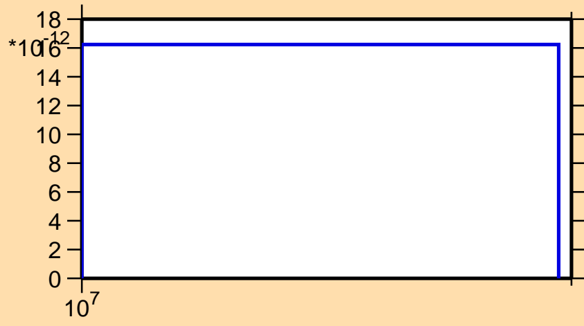
\sigma vs. E for ^{172}\text{Dy}(n,nd)
