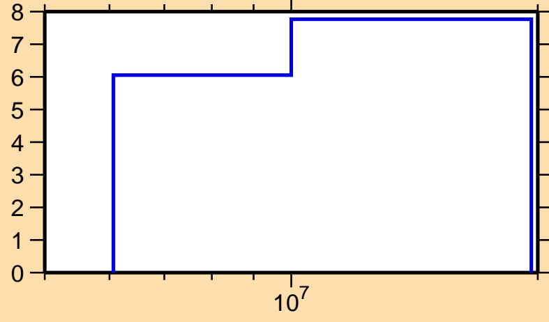
\Delta\sigma/\sigma vs. E for ^{172}\text{Dy}(n,\text{el.})
