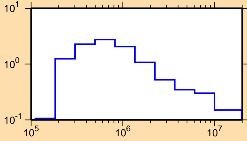
\sigma vs. E for ^{172}\text{Dy}(n,n_1)
