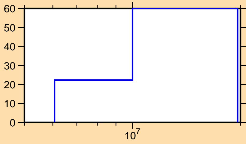
\Delta\sigma/\sigma vs. E for ^{172}\text{Dy}(n,2n)
