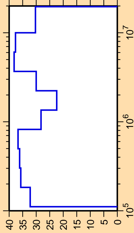
\Delta\sigma/\sigma vs. E for ^{172}\text{Dy}(n,n_1)
