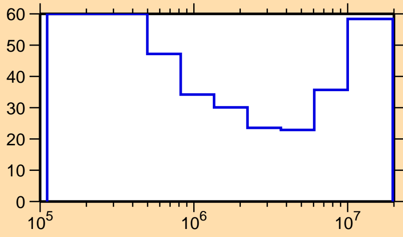
\Delta\sigma/\sigma vs. E for ^{172}\text{Dy}(n,n\text{cont.})
