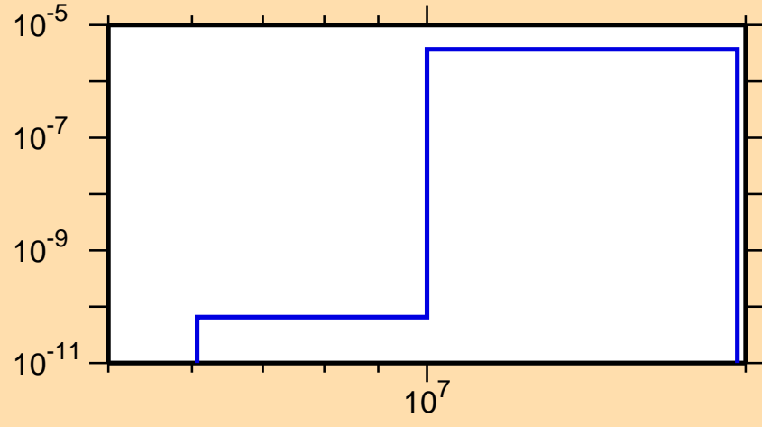
\sigma vs. E for ^{172}\text{Dy}(n,\alpha)
