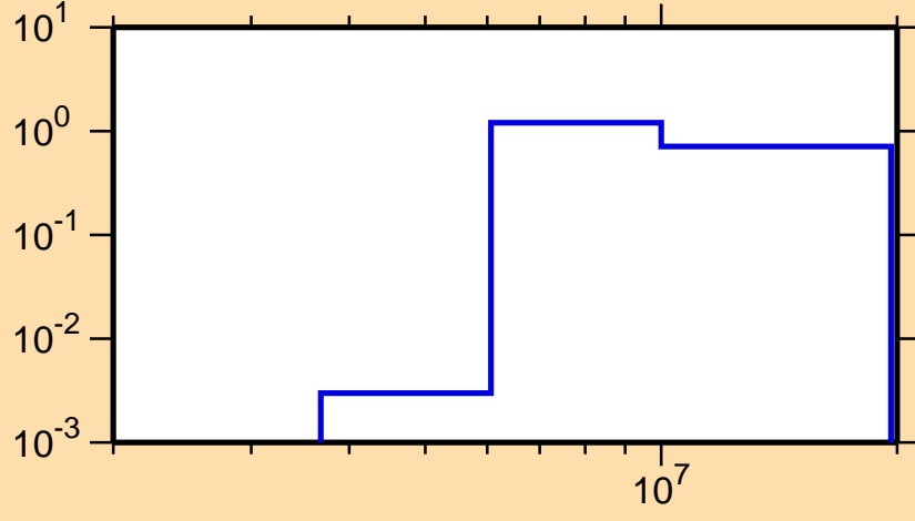
\sigma vs. E for ^{172}\text{Dy}(n,2n)
