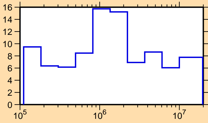
\Delta\sigma/\sigma vs. E for ^{172}\text{Dy}(n,\text{el.})
